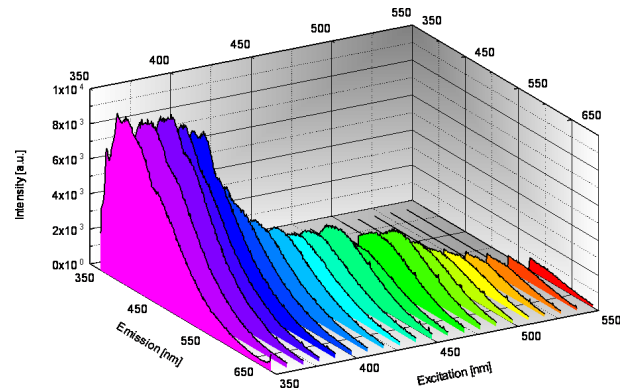
Fig. 1. The three-dimensional fluorescence spectrum of SEMTEX
