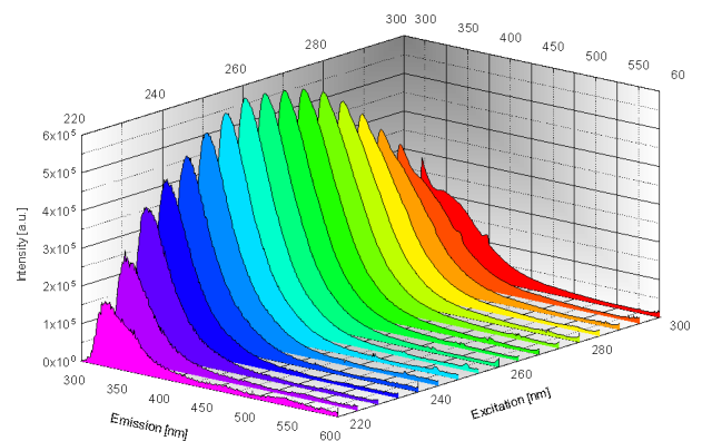
Fig. 2. Excitation and emission characteristics of tryptophan
