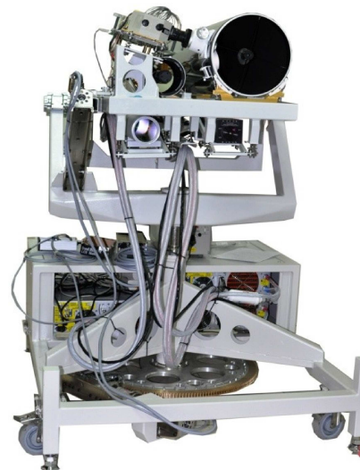
Fig. 3. Fluorescence/depolarization LIDAR for mid-range stand-off detection of the chemical and biological threats in the air
