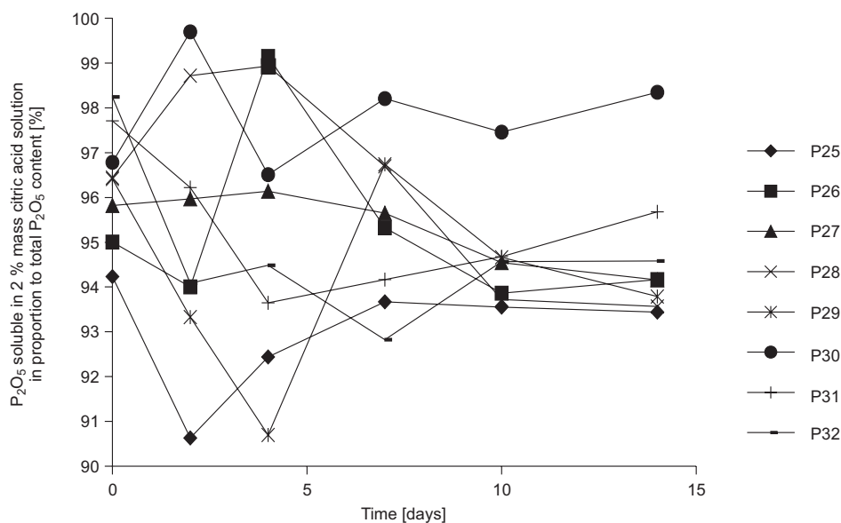
Fig. 8. Correlation P_2O_5 soluble in 2 % citric acid solution in ratio to total P_2O_5 content in time for products from 25 to 32
