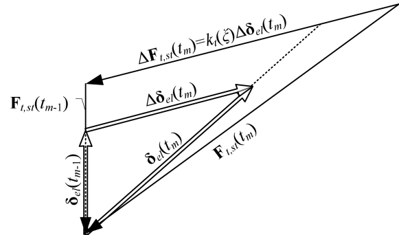
Fig. 7. The scheme for proving that the vectors \mathbf{F}_{t,st}(t_m) and \delta_{el}(t_m) are not parallel
