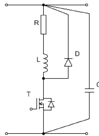
D – diode under test T – transistor switch Fig. 3. Circuit of the test system
