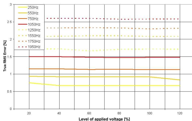
Fig. 6. Impact of the level of applied voltage of specific harmonic frequency on True RMS Error
