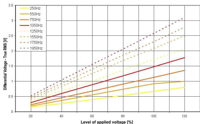
Fig. 5. Impact of the level of applied voltage on differential voltage
