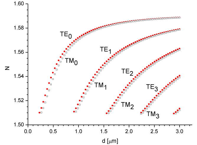
Fig. 1. Effective refractive indices as a function of the thickness d of the layer SU8
