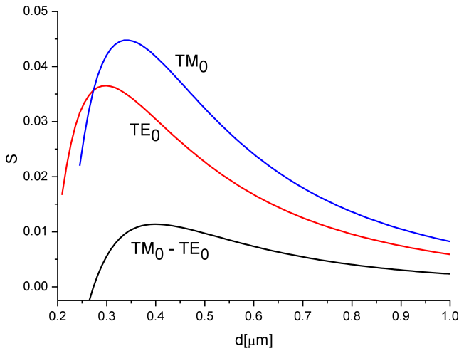
Fig. 2. Sensitivities as a function of the thickness of the waveguide layer concerning a single-mode waveguide
