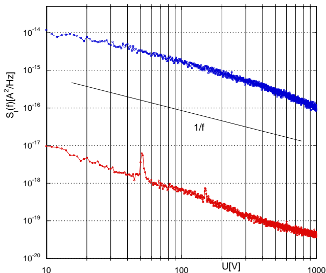
Fig. 14. Power spectral density of current noise for 440 V varistor samples (blue – poor quality, red – good quality samples).
