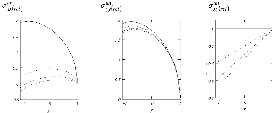
Fig. 4. Characteristic of stresses, \sigma_{xx(rel)}^{un} , \sigma_{yy(rel)}^{un} , \sigma_{xy(rel)}^{un} at \kappa = 0,3; 0,5; 0,75; 0,99 and \eta = 0,3; \xi = 0,1 .
