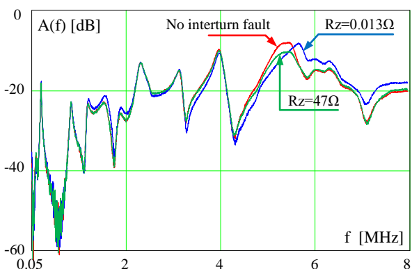
Fig. 6. Results of FRA magnitude response of the T2 winding without interturn fault and at two values of the shorting resistance R_z
