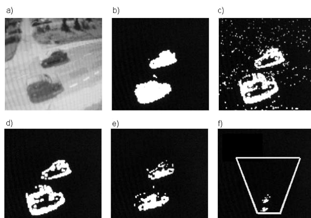
Fig. 6. Selected results of the sensor operation: a) input frame \mathbf{I}_t , b) mask \mathbf{m}_B , c) mask \mathbf{m}_S , d) mask \mathbf{m}_{HS} , e) output mask \mathbf{m}_V , f) final mask \mathbf{m}_V after the geometrical transformation, the original image boundaries are additionally marked
