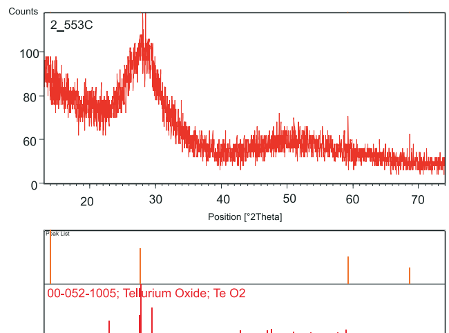
Fig. 2. Diffraction pattern of glass P2 exposed to 1 h thermal treatment in temperature of 553°C
