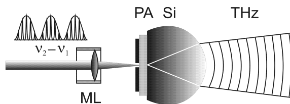
Fig. 13. Hyperhemispherical Si lens applied to a photoconductive antenna PA
