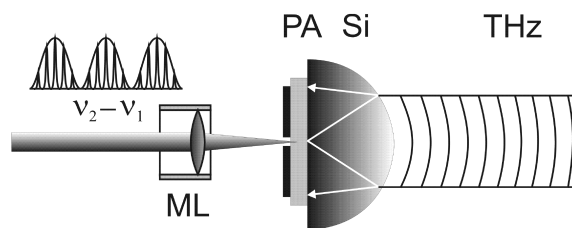
Fig. 12. Photoconductive antenna PA fixed to a hemispherical lens Si. ML – microscopy lens
