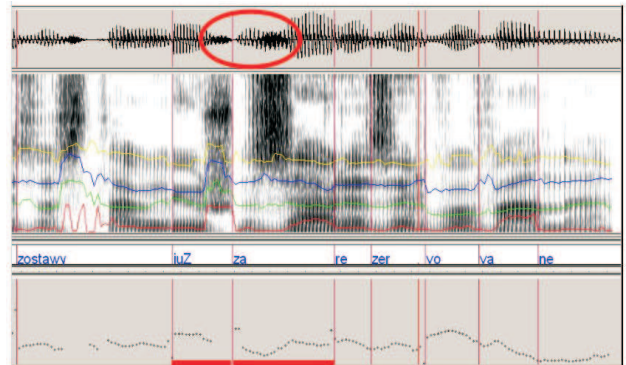
Fig. 5. Selecting units based on matching feature specifications of both the target and the adjacent units can prevent poor concatenations such as the one between the fricatives [Z] and [z] (marked by the red ellipse)
