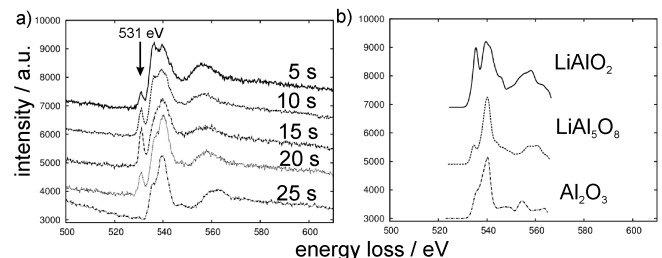
Fig. 19. Time-resolved ELNES of \gamma - \text{LiAlO}_2 : a) Experimental O-K edge spectra acquired at a focused electron beam of 1 nm in diameter at 200 kV accelerating voltage at different irradiation time; b) simulated ELNES of O-K edge for different phases
