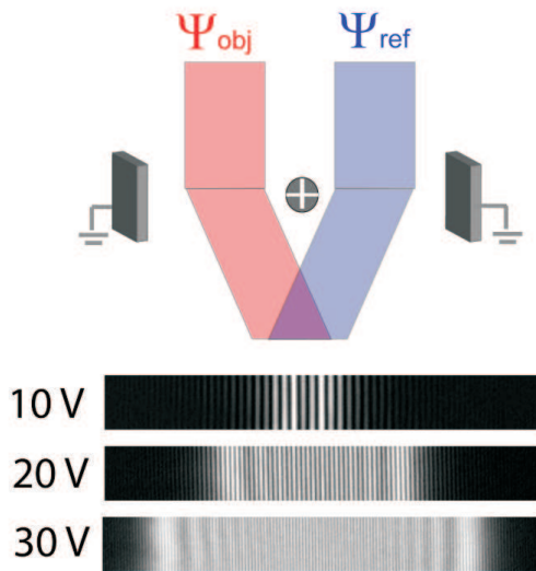
Fig. 25. Basic principle of off-axis electron holography
