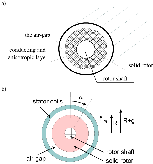
Fig. 2. Cylindrically shaped electromechanical converter – a) its cross section – b)
