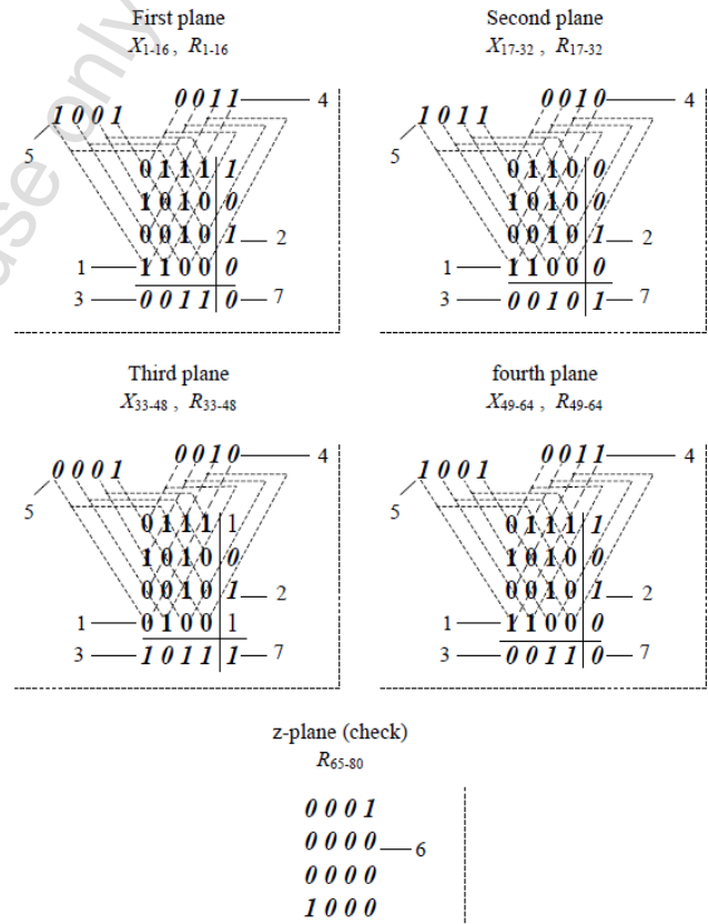
Fig. 1. The principle of check symbols formation by three-dimensional linear iterative code with double incorporated diagonal checks
