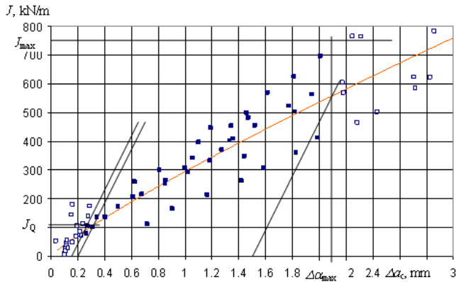
Fig. 3. Experimental fracture toughness data for “V”- type weld specimens welded by electrodes CT-36 and averaged J - R curve (line)
