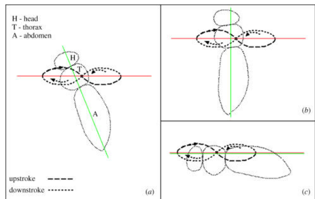
Fig. 8. Generic kinematics of insect in hover: the wing tip traces a 'figure-of eight', when seen from the insect side. The angle between the insect body axis (green) and the stroke plane (red) is constant. Typically, (a) the angle is steep; (b) one extreme: the angle is \pi/2 ; (c) the other extreme: the angle is zero (see Żbikowski and Galiński [48]).
