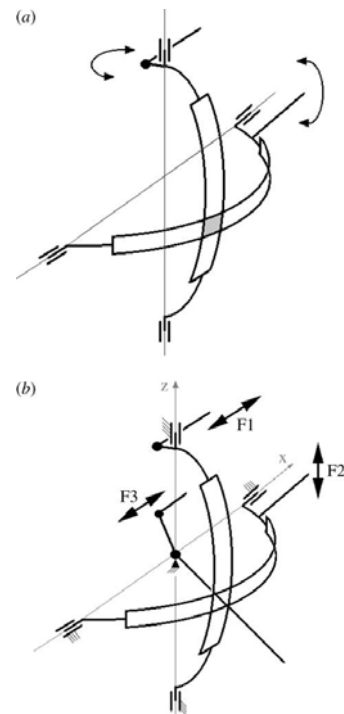
Fig. 9. Spherical double Scotch yoke: (a) kinematic diagram; (b) concept of the associated flapping mechanism (cf. Zbikowski and Galinski [48])
