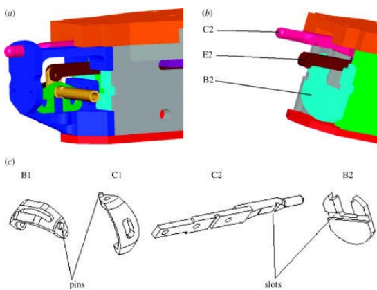
Fig. 11. Details of the driving components [48]
