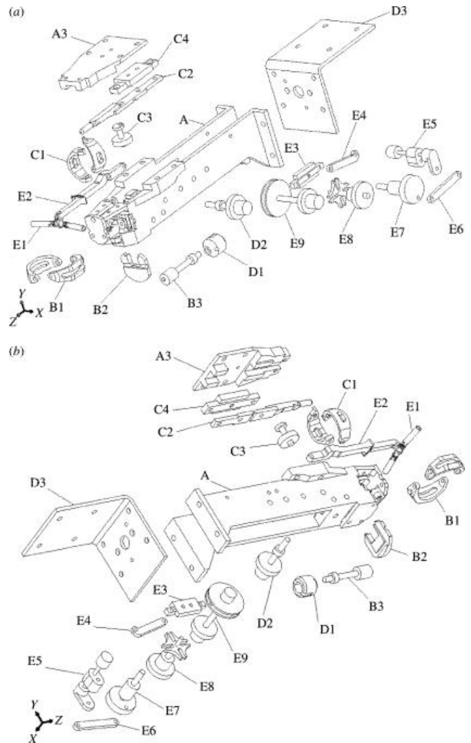
Fig. 12. The exploded view of the complete mechanics
