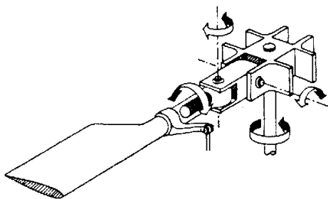
Fig. 7. Articulated joints of a helicopter main rotor
