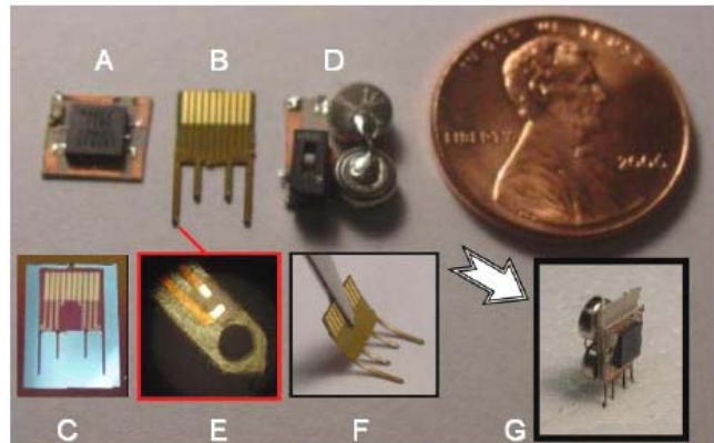
Fig. 22. The microsystem including microprocessor (A), flexible probe (B), silicon probe (C) and battery unit for power (D), the close-up view of the tip in (E) with the hole for muscle growth, the flexibility of the probe (F) and the assembled system (G) (cf. [5]).
