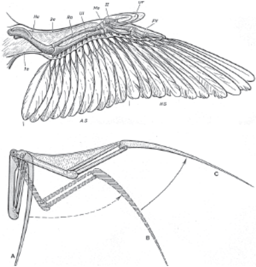
Fig. 6. Bird wing hinges anatomy, and wing folding
