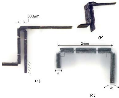
Fig. 16. Designed by prof. Wood MAV transmission system, top view (a) and isometric view (b). The slider-crank for coupling actuator motion to the prismatic input of the transmission is shown in (c) (cf. 44)
