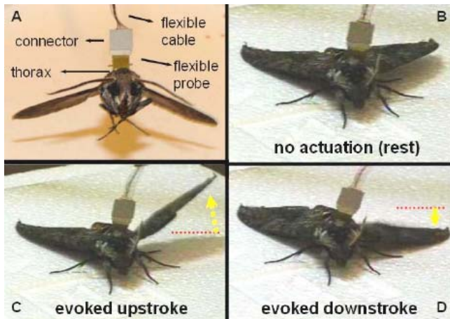
Fig. 23. The evoked up- and downstroke of a “single” wing obtained by applying 5V pulses to the indirect flight muscles (snapshots from the recorded movie). Under natural conditions, moths flap both wings together (cf. [5])
