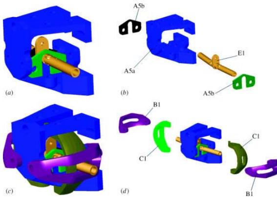
Fig. 10. Practical realization of spherical double Scotch yoke (Zbikowski and Galinski [48])
