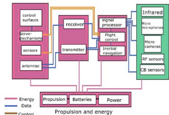
Fig. 1. Integration of MAV systems [22]
