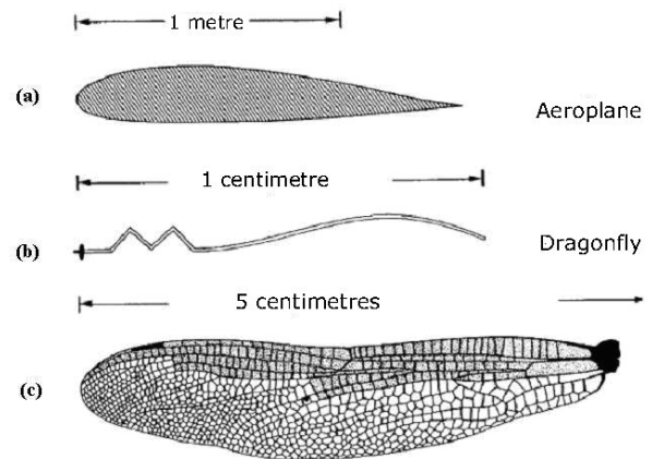
Fig. 19. Comparison of aircraft and dragonfly wing cross-section (airfoil) a) aircraft airfoil, b) dragonfly wing cross-section, c) dragonfly wing shape
