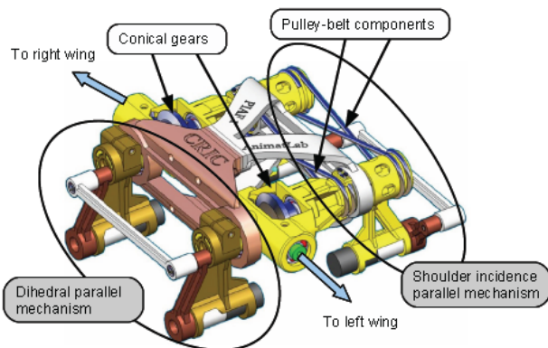
Fig. 14. ROBUR wing propulsion gearbox
