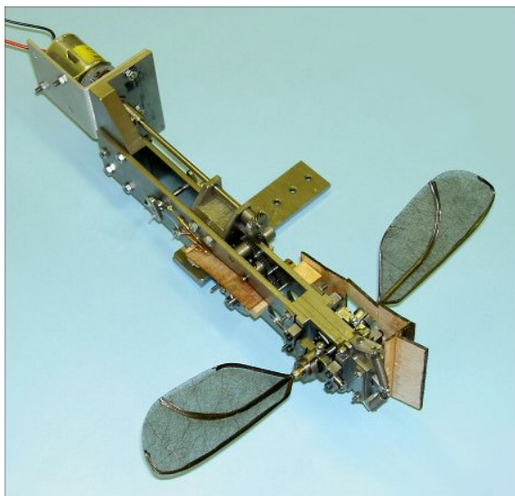
Fig. 13. General view of the Dr. Zbikowski complete mechanism
