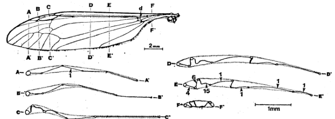
Fig. 20. Folds created on cross-section of a wing generate vortices causing, transformation of wing plate into effective airfoil
