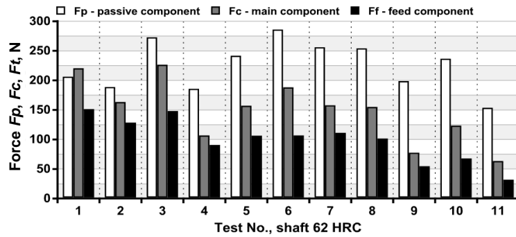
Fig. 12. Comparison between components of the total cutting force in turning of hardened cold work tool steel (X165CrV12) with the CBN tool (62 HRC)
