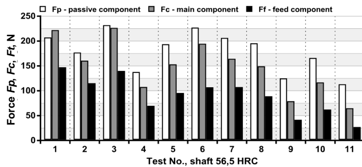
Fig. 11. Comparison between components of the total cutting force in turning of hardened cold work tool steel (X165CrV12) with the CBN tool (56.5 HRC)
