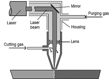
Fig. 2. Main principle of laser cutting
