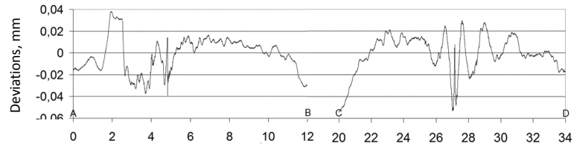
Fig. 6. Deviations of measured contour from the theoretical (design) shape. Low carbon steel, v_f = 1800 mm/m
