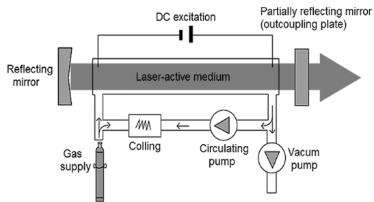
Fig. 1. Design of laser device
