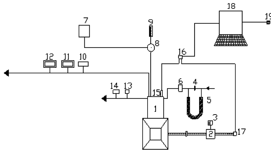
Fig. 2. Experimental Set-up
