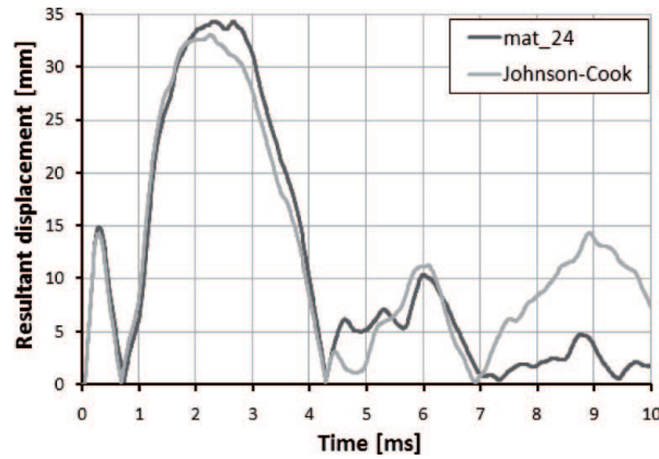
Fig. 18. Resultant displacement of “representative location 1” on the skin
