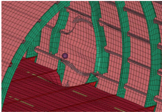
Fig. 12. Fuselage deformation (charge between frames; t = 10\text{ms} )
