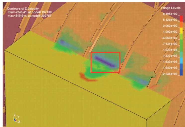
Fig. 8. The Euler domain – non-physical disturbance of the fluid
