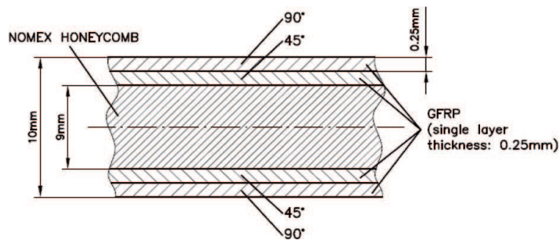
Fig. 3. Fuselage floor cross section
