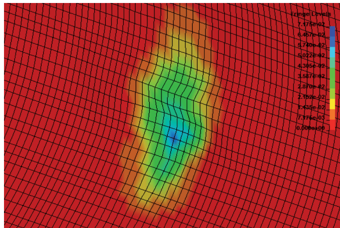
Fig. 13. Skin – plastic strain, max 7.2% (charge between frames; t = 10\text{ms} )
