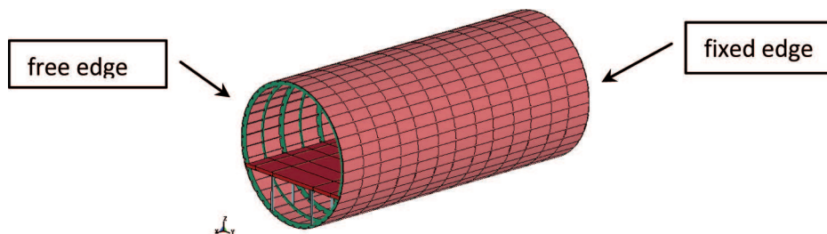
Fig. 4. Boundary conditions
