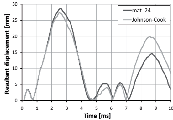
Fig. 19. Resultant displacement of “representative location 2” on the skin
