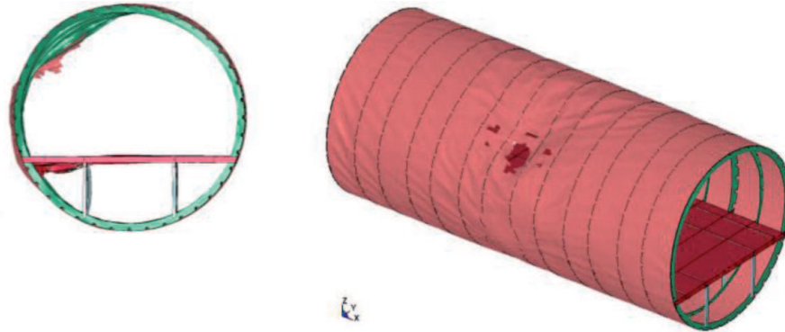
Fig. 10. Model 2 – deformation of the fuselage at t = 10\text{ms}
