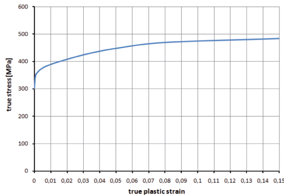
Fig. 2. AL2024-T3 stress-strain characteristic
