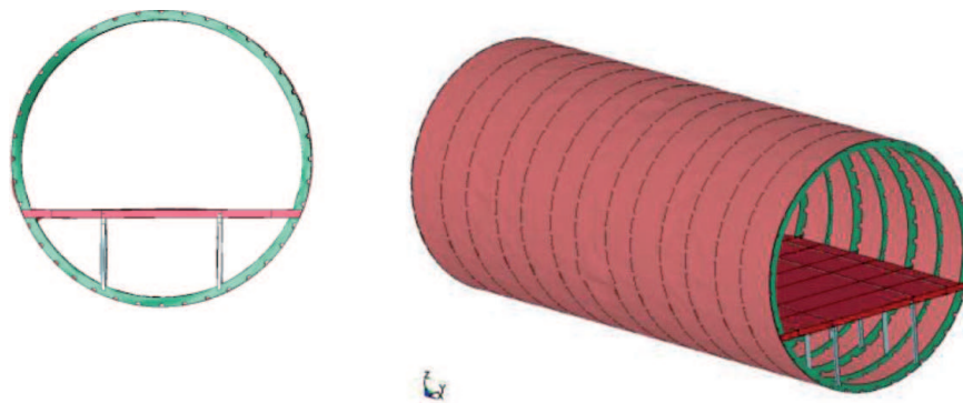
Fig. 11. Model 3 – deformation of the fuselage at t = 10\text{ms}
