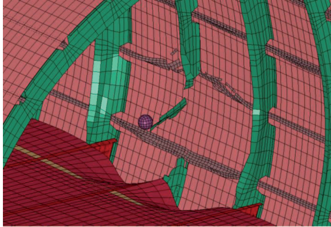
Fig. 14. Fuselage deformation (charge opposite to a frame; t = 10\text{ms} )
