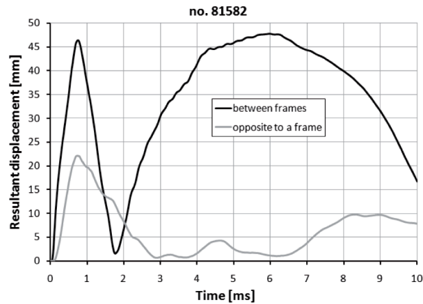
Fig. 17. Resultant displacement (modulus) of the node from Fig. 16
