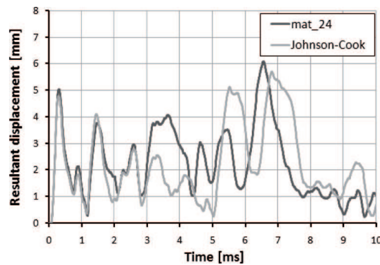
Fig. 20. Resultant displacement of “representative location 3” on the skin
