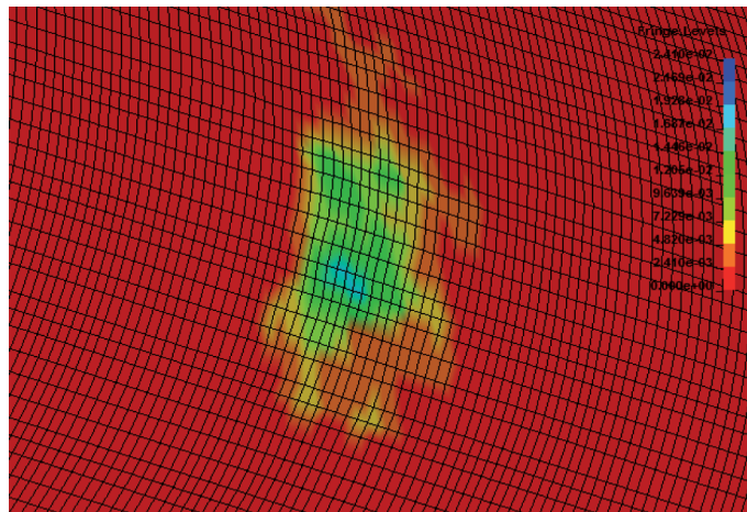
Fig. 15. Skin – plastic strain, max 2.4% (charge opposite to a frame; t = 10\text{ms} )
