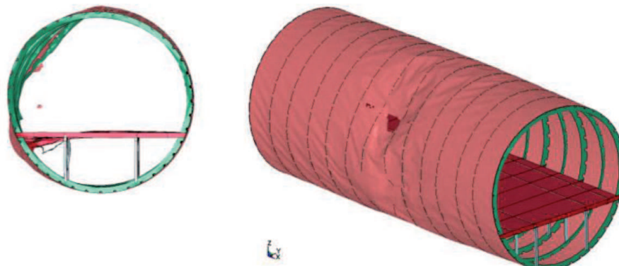
Fig. 9. Model 1 – deformation of the fuselage at t = 10\text{ms}
