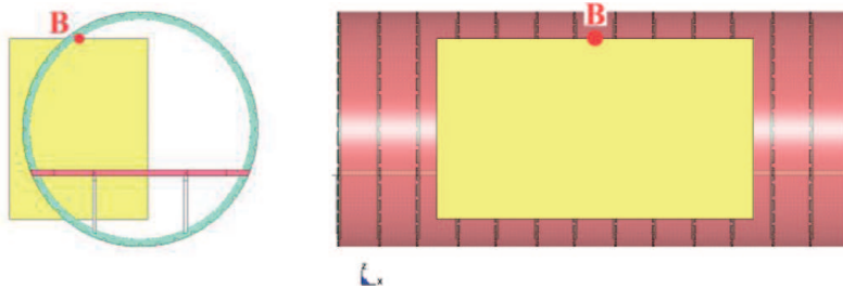
Fig. 6. Model 2 – dimensions of the Eulerian mesh: 1765mm×2305mm×4030mm
