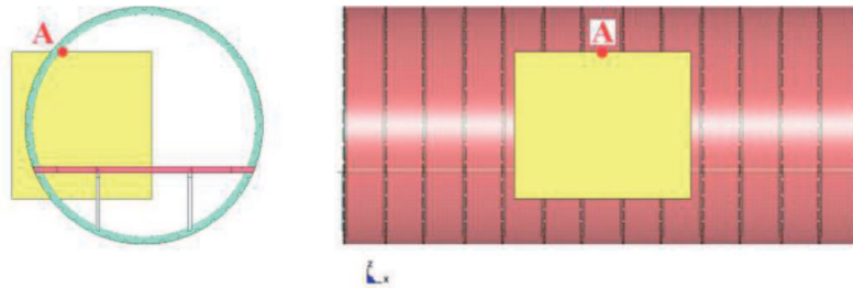
Fig. 5. Model 1 – dimensions of the Eulerian mesh: 1765mm×1855mm×2230mm
