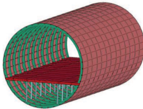
Fig. 1. Geometry of the FE model (it is NOT the mesh)
