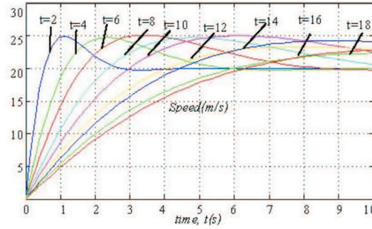
Fig. 3. Step response of the closed loop system for different rise times, from left to right t_r=2,4,6,8,10,12,14,16,18 sec, when step input is 20 m/s
