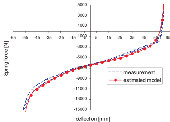
Fig. 2. Spring force as function of deflection of the shock-absorber assembly
