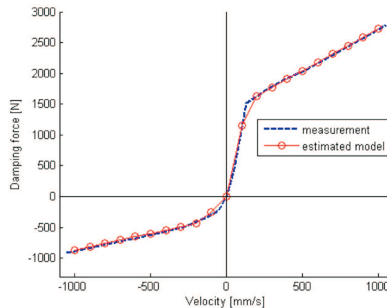
Fig. 3. Steady-state damping force as function of shock-absorber velocity
