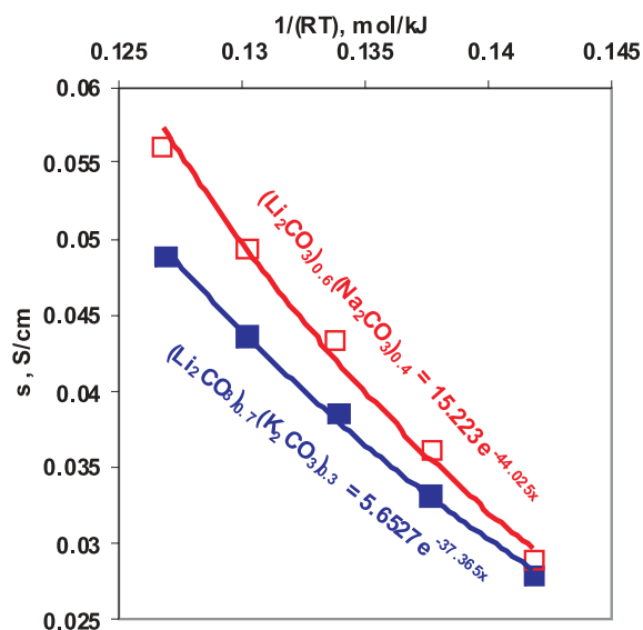
Figure 8. Temperature dependence of ionic conductivity for molten carbonates.
