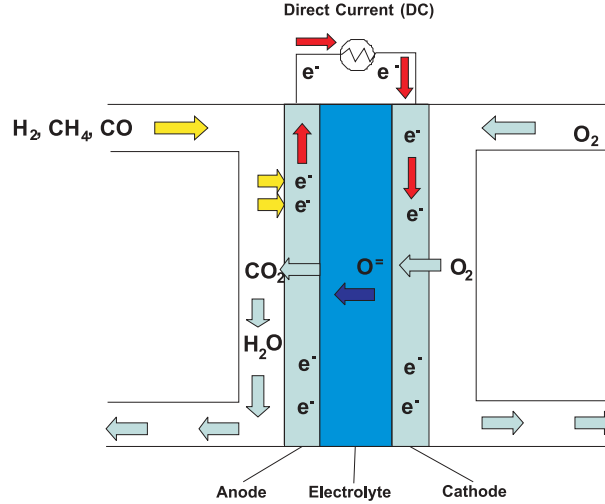
Figure 4. Working principles of SOFC.
