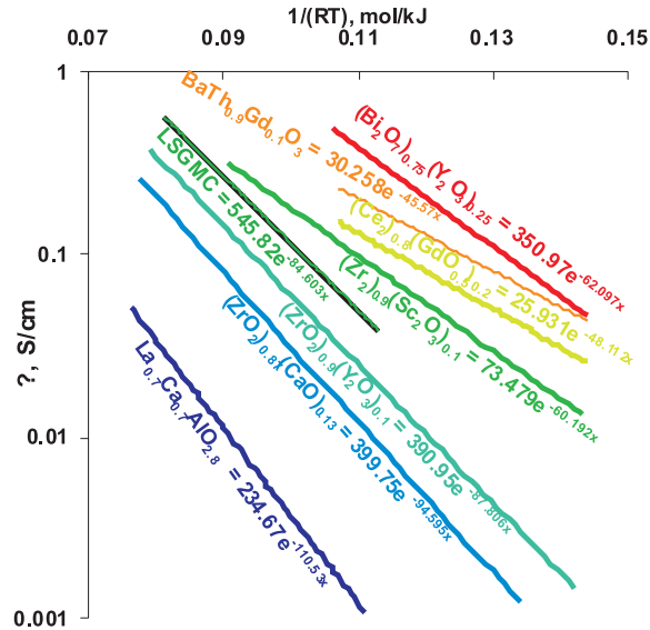
Figure 6. Temperature dependence of ionic conductivity for solid oxides.
