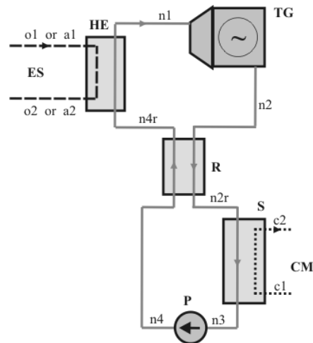
Figure 2. ORC power plant with internal regeneration (CM – cooling medium, ES – energy source, HE – supercritical heat exchanger, P – pump, R – regenerator, TG – turbogenerator).
