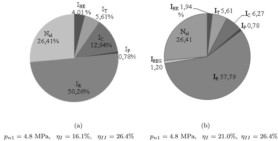
Figure 4. Split of exergy rates in the supercritical ORC power plant (a) without regeneration, (b) with regeneration.
