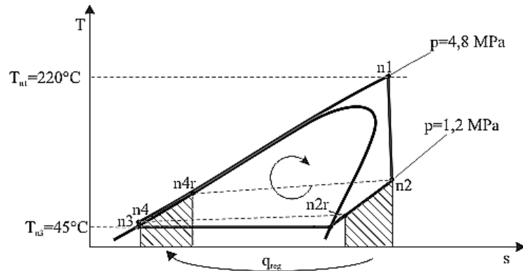
Figure 3. Supercritical ORC power plant with internal regeneration for the vapour pressure p_{n1} = 4.8 MPa.
