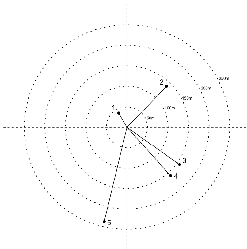
Fig. 4. Direction and range of missiles from LPG tank explosion – 2.
