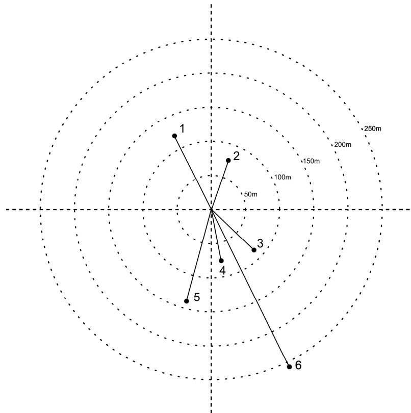
Fig. 3. Direction and range of missiles from LPG tank explosion – 1.
