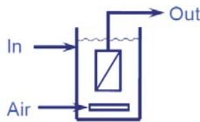
Figure 2. Submerged membrane bioreactors [1].
