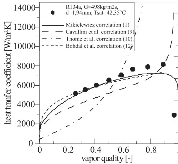
Figure 6. Comparison of heat transfer coefficient for R134a in relation to experimental data due to Bohdal et al. (2011), d = 1.94 \text{ mm} , G = 498 \text{ kg/m}^2\text{s} , T_{sat} = 42.4 \text{ }^\circ\text{C} .
