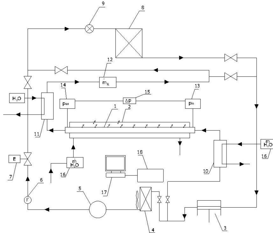
Figure 2. Schematic diagram of the experimental facility: 1 – measuring section of the pipe minichannel, 2 – water channel, 3 – refrigeration compressor installation, 4 – condenser chilled with air, 5 – container of refrigerant liquid, 6 – filter-dryer of refrigerant, 7 – electromagnetic valve, 8 – lamelled air cooler, 9 – expansion valve that feeds the cooler, 10 – heat exchanger to collect refrigerant's superheat, 11 – subcooler of refrigerant's liquid, 12 – electronic flowmeter of refrigerant, 13 – refrigerant's pressure pickup on the inlet to the measuring section, 14 – refrigerant's pressure pickup on the outlet to the measuring section, 15 – refrigerant's differential pressure transducer, 16 – water electronic flowmeter, 17 – computer, 18 – data processing system, F – filter.
