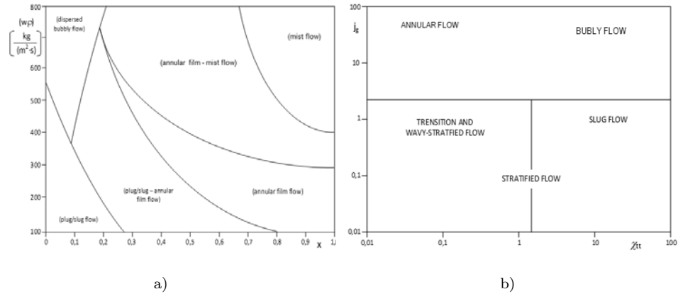
Figure 1. Maps of two-phase flow structures in the condensation process of R134a refrigerant in minichannels according to: a) Coleman and Garimella [8], b) Cavallini et al. [5].
