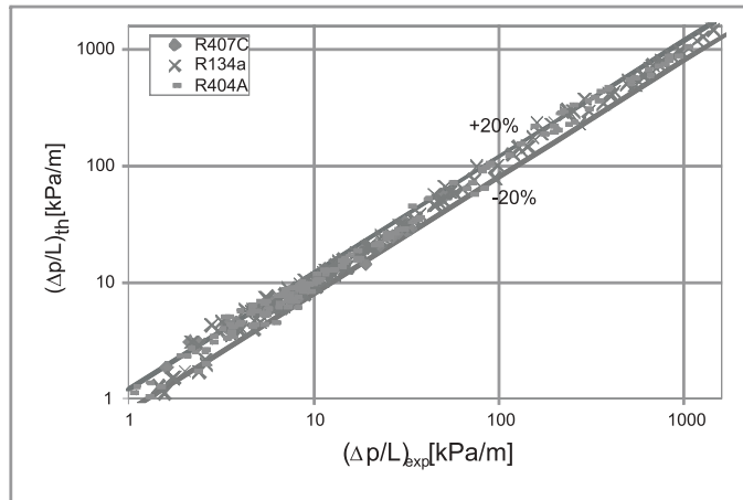
Figure 12. Comparison of the results of experimental investigations and the results of calculations from the correlation (1) concerning the local pressure drop in the flow of R134a, R404A and R407C refrigerants during condensation in pipe minichannels with internal diameters d = 0.31\text{--}3.3 mm.
