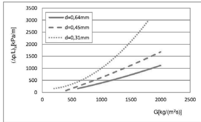
Figure 8. Comparative setting-up of the results of experimental investigations of dependence (\Delta p/L)_a upon the mass flux density, G , during the condensation of refrigerant R134a in pipe minichannels with diameters d = 0.31 – 0.64 mm.
