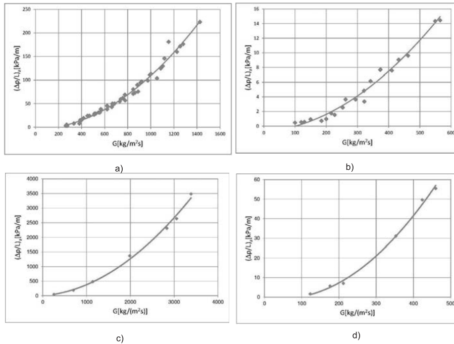
Figure 4. Graphical interpretation of an experimental dependence of flow resistance, (\Delta p/L)_a , from the mass flux density, G , during condensation in a pipe minichannel: a) R134a, d = 1.40 mm, b) R134a, d = 3.30 mm, c) R407C, d = 0.31 mm; d) R407C, d = 0.98 mm.
