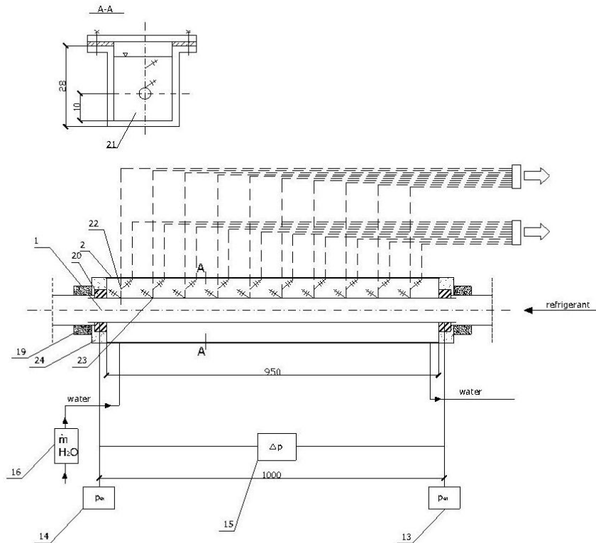
Figure 3. Schematic diagram (sectional view) of the measuring section of the pipe minichannel; 19c copper pipe 8/ 10 mm, 20 – pipe connector, 21 – pipe minichannel refrigeration system, 22 – connector of thermocouple wires of water temperature thermocouples, 23 – connector of thermocouple wires of minichannel surface thermocouples, 24 – isolation, K – thermocouples (the remaining denotations as in Fig. 2).
