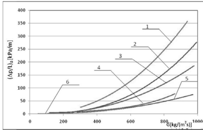
Figure 7. Cumulative setting-up of experimental dependence (\Delta p/L)_a upon the mass flux density, G , for refrigerant R134a during its condensation in pipe minichannels with internal diameters d = 0.98 – 3.30 mm: 1 – d = 0.98 mm, 2 – d = 1.40 mm, 3 – d = 1.60 mm, 4 – d = 1.94 mm, 5 – d = 2.30 mm, 6 – d = 3.30 mm.
