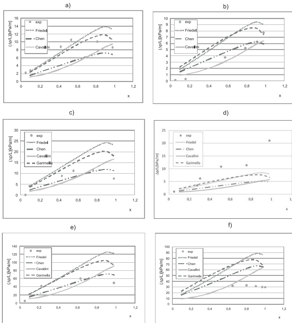
Figure 11. Comparison of experimental investigations of dependence (\Delta p/L)_x upon the quality, x , with the results of calculations according to correlations proposed by other authors during condensation of R134a and R404A refrigerant in minichannels with the following diameters: a) R134a, d = 2.3 mm, G = 321 kg/m 2 s, T_s = 30 °C; b) R404A, d = 2.3 mm, G = 321 kg/m 2 s, T_s = 43 °C; c) R134a, d = 1.94 mm, G = 376 kg/m 2 s, T_s = 40 °C; d) R404A, d = 1.94 mm, G = 376 kg/m 2 s, T_s = 33 °C; e) R134a, d = 1.4 mm, G = 541 kg/m 2 s, T_s = 45 °C; f) R404A, d = 1.4 mm, G = 866 kg/m 2 s, T_s = 40 °C.
