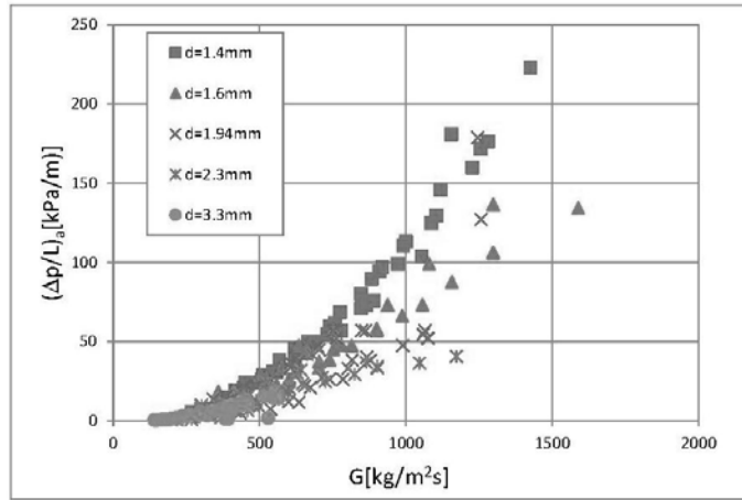
Figure 5. Setting-up of the experimental results of the condensation of R404A refrigerant in pipe minichannels with internal diameters d = 1.4\text{--}3.3 mm.
