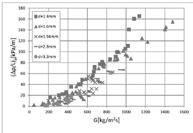
Figure 6. Comparative setting-up of the results of experimental investigations of the condensation of R134a refrigerant in pipe minichannels with internal diameters d = 1.4\text{--}3.3 mm.
