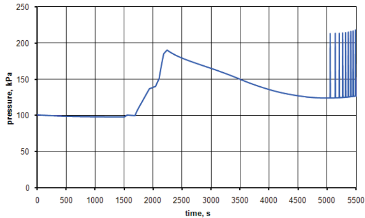
Figure 7. Pressure trend under the containment dome considering the local combustion effects.
