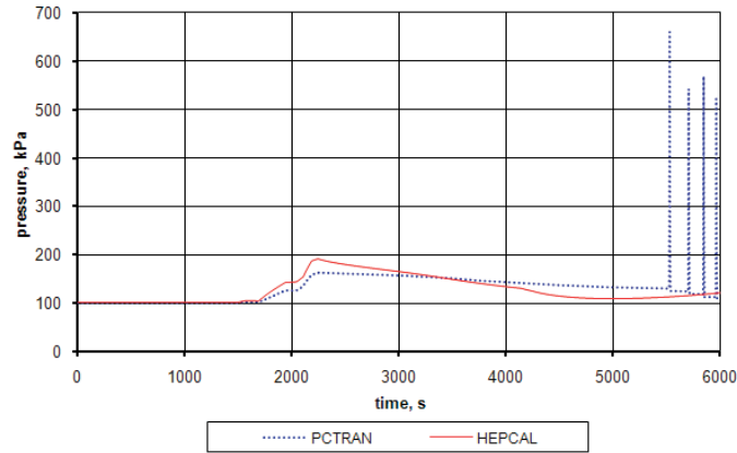
Figure 4. Pressure trend inside the containment during the analyzed accident.
