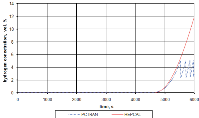
Figure 5. Hydrogen concentration inside the containment during the analyzed accident.
