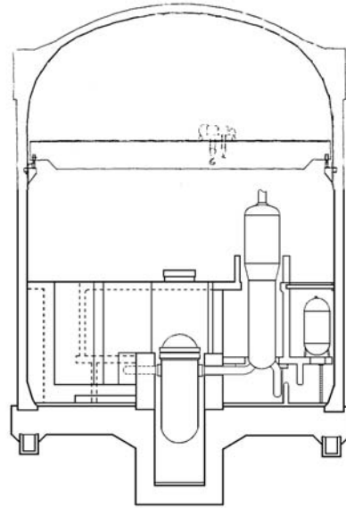
Figure 1. Sketch of the standard second generation PWR containment [10].
