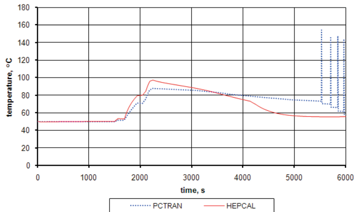
Figure 3. Temperature trend inside the containment during analyzed accident.
