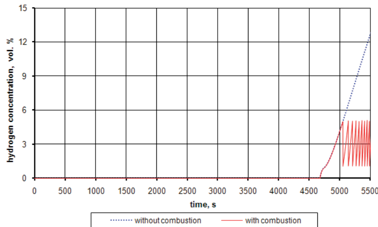
Figure 6. Hydrogen concentration within the leakage zone.
