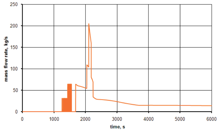
Figure 2. Mass flow rate of the coolant leakage (according to simulation made using the PCTRAN).
