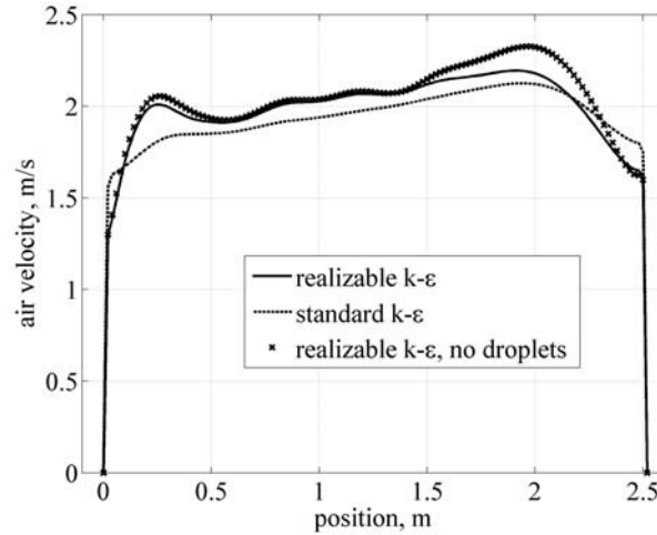
Figure 5. Profiles of velocity at the inlet to the fill for standard k\text{-}\epsilon , realizable k\text{-}\epsilon and realizable k\text{-}\epsilon omitting the flow of water droplets in the rain zone.
