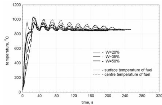
Figure 18. An example of temperature changes of coal*-water suspension during its cyclic combustion in air ( 10s_A/10s_N ). * the mixture 50%/50% of hard coal and coal slurry (Sobieski mine)
