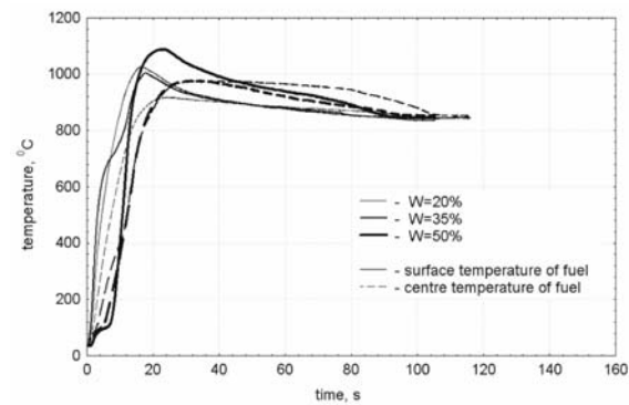
Figure 16. An example of temperature changes of coal*-water suspension during its continuous combustion in air. * the mixture 50%/50% of hard coal and coal slurry (Sobieski mine), W – moisture content, %.
