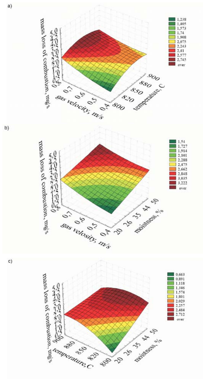
Figure 10. Relation between: a) temperature in the combustion chamber and gas velocity, b) gas velocity and moisture of suspension, c) temperature in the combustion chamber and moisture of suspension and the mass rate of fuel combustion during cyclic combustion 10s_A/10s_N ( s_A/s_N – time combustion in air/time residence in nitrogen); hard coal dust (mine Sobieski): below 250 \mu\text{m} .
