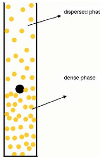
Figure 23. Subregions in the fluidized bed.
