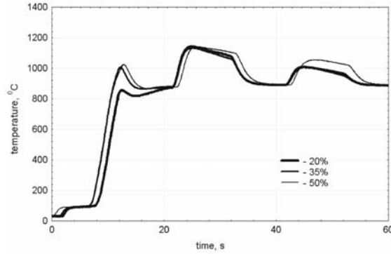
Figure 8. Relation between moisture of suspension (20%, 35%, 50%) and temperature of hard coal-water suspensionl (mine Sobieski) during cyclic combustion 10s_A/30s_N ( s_A/s_N – time combustion in air/time residence in nitrogen).
