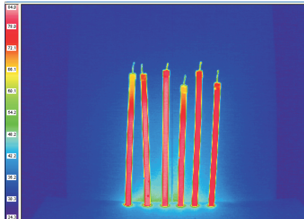
Figure 9. Development of surface temperature of heat pipe at heating time 15:11 min.
