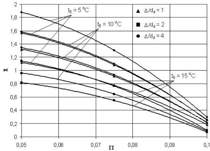
Figure 3. The ejection ratio \chi for the refrigerating system with a two-phase ejector as the first compression stage.
