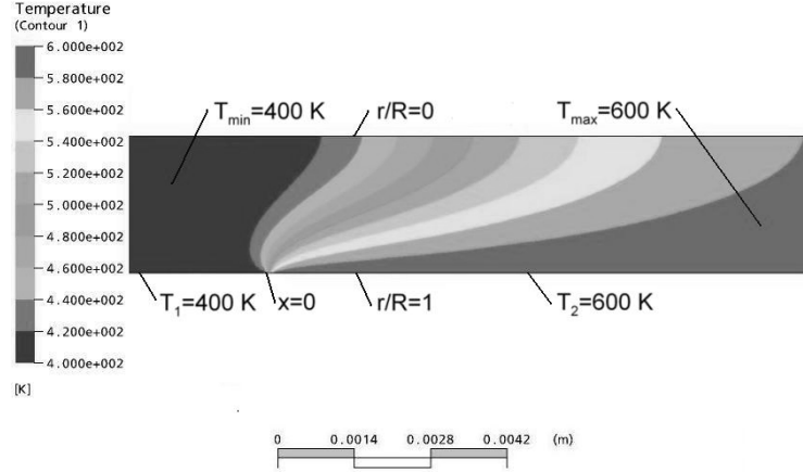
Figure 3. Temperature distribution in fluid for laminar flow using the mesh C, K.
