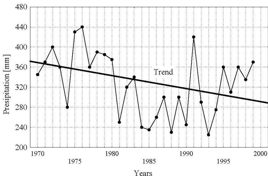
Fig. 5. Changes and trend of the sum of precipitation during the 1970–2000 period (SLAVOV and ROUSSEVA, 2000)
