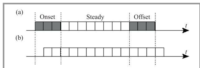
Fig. 7. Segment evaluation by TIA/EIA-136-250: (a) ideal signal, (b) testing signal.
