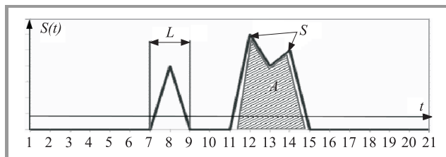
Fig. 4. Segment features.
