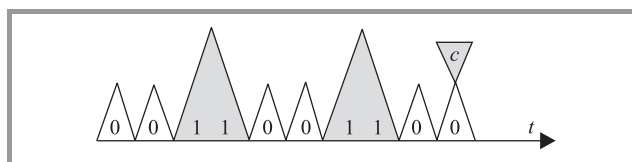
Fig. 3. Extrema-based segmentation: 0 – noise segment, 1 – speech segment, c – current position.
