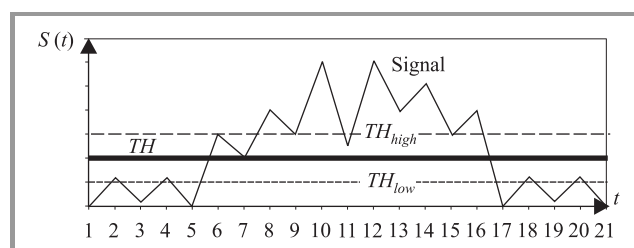
Fig. 1. Threshold-based segmentation.
