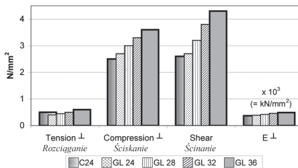
Fig. 3. Axial (perpendicular to the grain) and shearing strengths, modulus of elasticity for solid timber C24 and glulam timber
