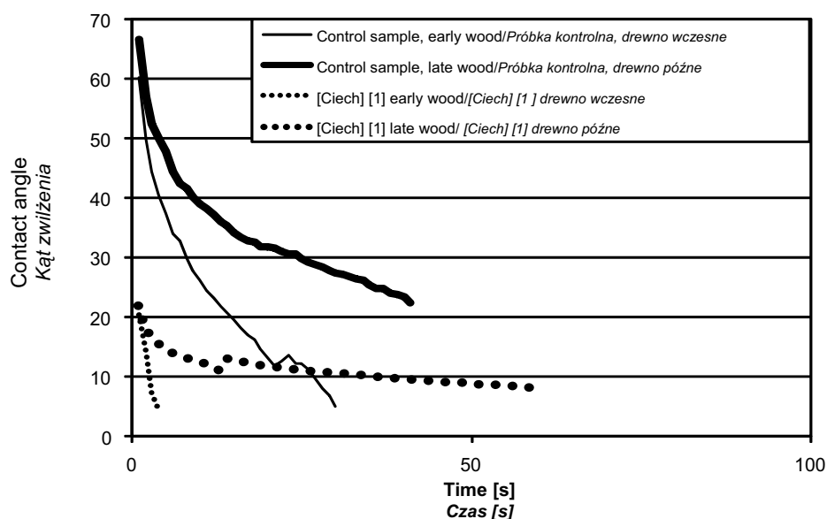
Fig. 3. Contact angles determined on the tangential section of the control samples and the samples treated with [Ciech] [1]
