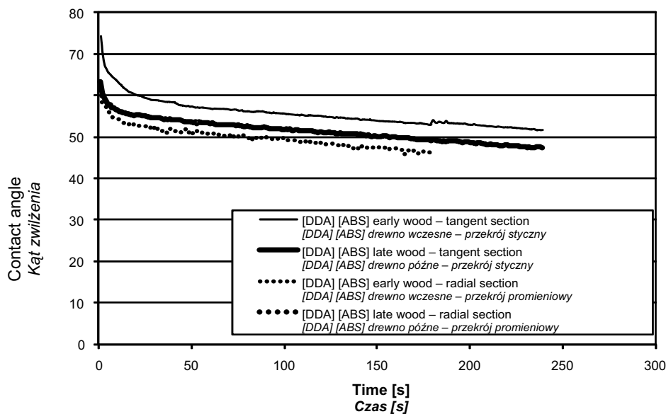
Fig. 4. The contact angles of early wood and late wood protected with [DDA] [ABS] depending on the wood section
