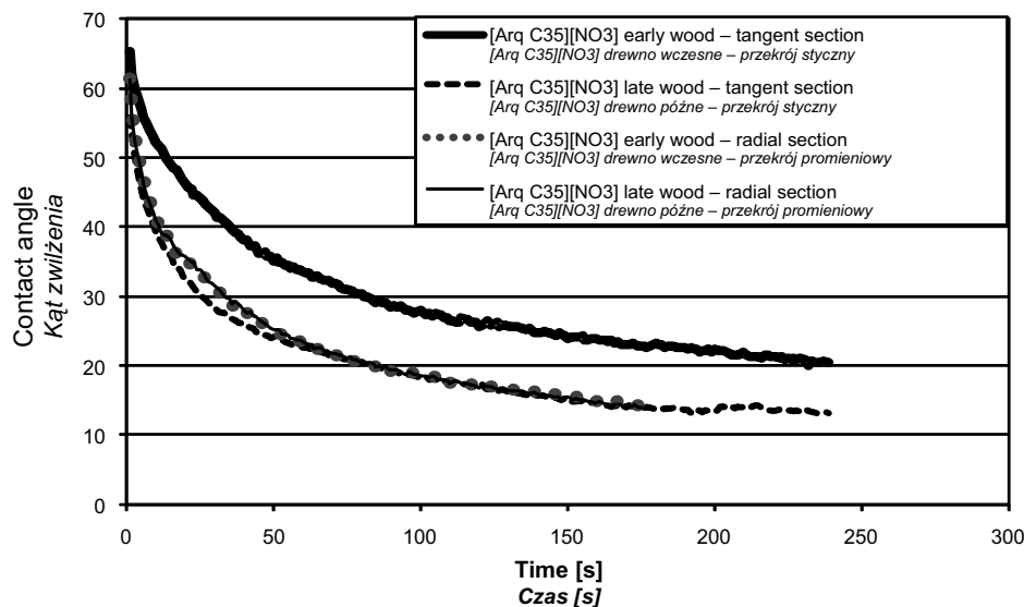
Fig. 4. The contact angles of early wood and late wood protected with [Arq C35] [NO 3 ] depending on the wood section
