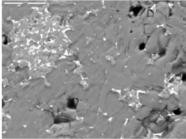
Fig. 5. Varistor with MnO-modified \text{Bi}_2\text{O}_3 . Marker 20 \mu\text{m} .
