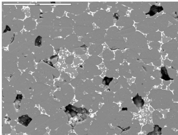
Fig.1. SEM image of the polished surface of ZnO varistor.
