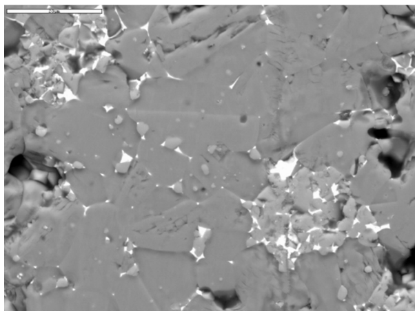
Fig. 6. Varistor with PbO-modified \text{Bi}_2\text{O}_3 . Marker 20 \mu\text{m} .
