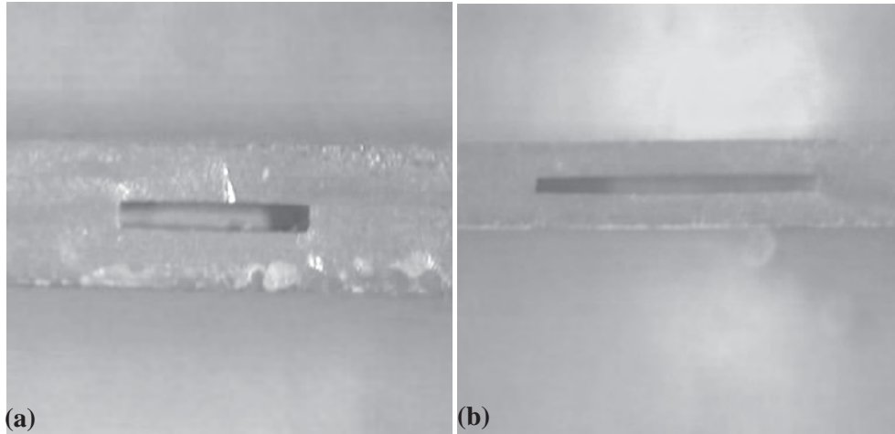
Fig. 1. Optical microscope image: (a) size of the chamber 2 x 2 mm 2 ; (b) size of the chamber 5 x 5 mm 2 .
