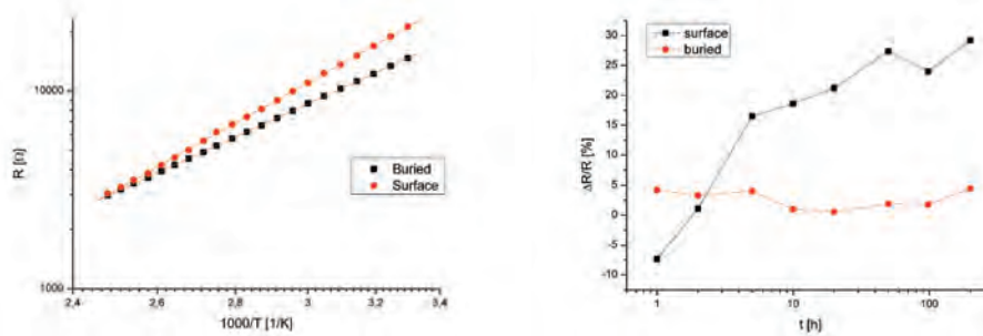
Fig. 5. (a) The temperature characteristics of resistance for ESL NTC-2114 thermistor composition, (b) long-term stability of ESL NTC-2114 thermistor composition.
