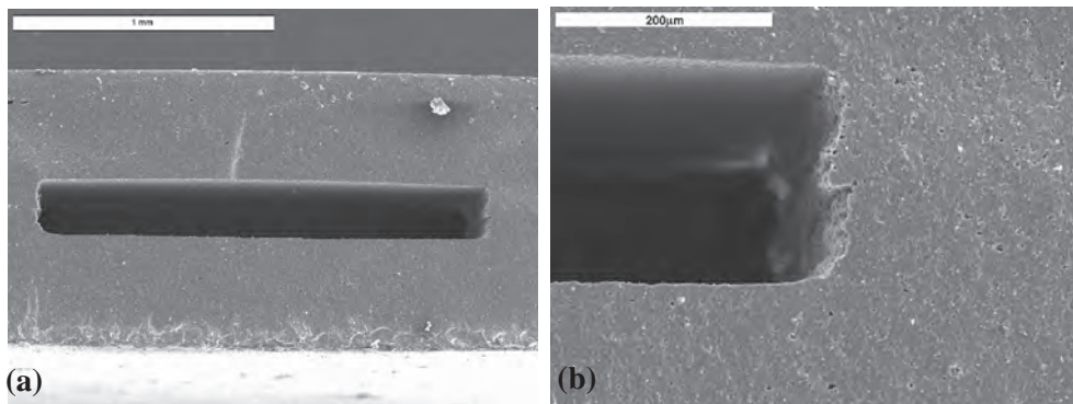
Fig. 2. Scanning Electron Microscope image of the tape bonding quality of the chamber area 2x2 mm 2 : a) lower zoom; b) larger zoom.
