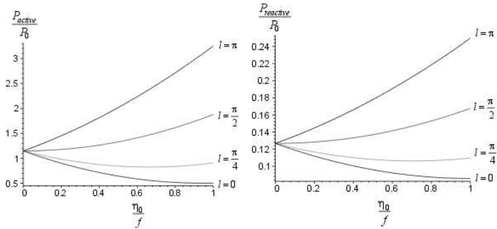
Fig. 2. The active and reactive sound power plotted in terms of parameter \eta_0/f for \beta = 15 , \delta = 0.5 and for some values of the differences between the phases associated with the excitations.
