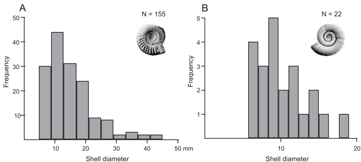
Fig. 6. Size-frequency histogram of A — Parkinsonia and B — Nannolytoceras shells — the most common ammonites in the concretions investigated; juvenile specimens dominate
