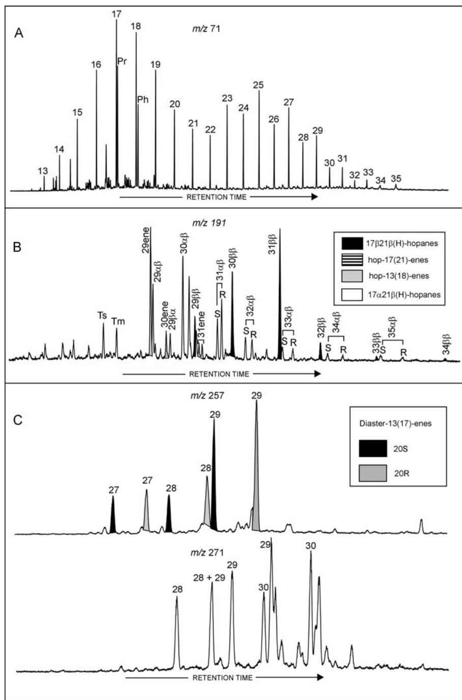
Fig. 3. Distribution of A — n -alkanes and isoprenoids (numbers indicate chain length of n -alkanes, Pr — pristane, Ph — phytane); chromatographic column: DB-5MS; B — pentacyclic triterpenoids; column: DB-5MS; C — diaster-13(17)-enes ( m/z 257) and 4 \beta -methyldiaster-13(17)-enes ( m/z 271); column: DB-17MS from the Bajocian carbonate concretions
