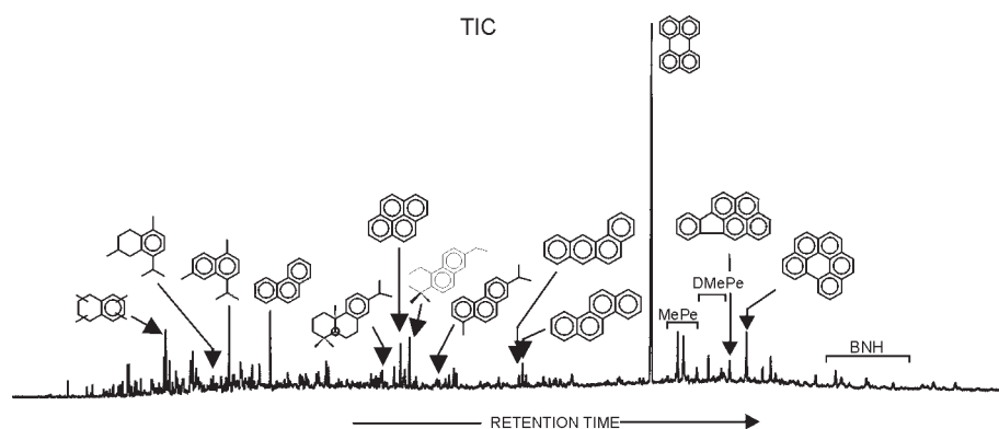
Fig. 4. Total ion chromatogram (TIC) of the aromatic fraction from the Bajocian Konzentrat-Lagerstätte-type carbonate concretions
