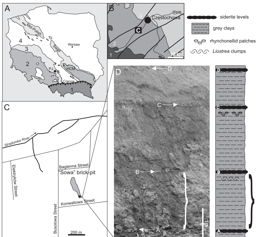
Fig. 1. A — simplified geological map of Poland without Cenozoic cover: the asterisk — area investigated, 1 — Carpathian Orogen, 2 — Pre-Jurassic rocks, 3 — Jurassic rocks, 4 — Cretaceous rocks, PJ — Polish Jura, HCM — Holy Cross Mts.; B — geological map of the study area: 1 — Lower Jurassic, 2 — Middle Jurassic, 3 — Upper Jurassic; C — localization sketch of “Sowa” brick-pit at Kawodrza Górna (adopted from Matyja and Wierzbowski, 2000), the asterisk — face investigated; D — the photograph of the section investigated with indicated siderite levels (A–D), with schematic section to better show their position, the brackets indicate the interval of fossil-rich carbonate concretions
