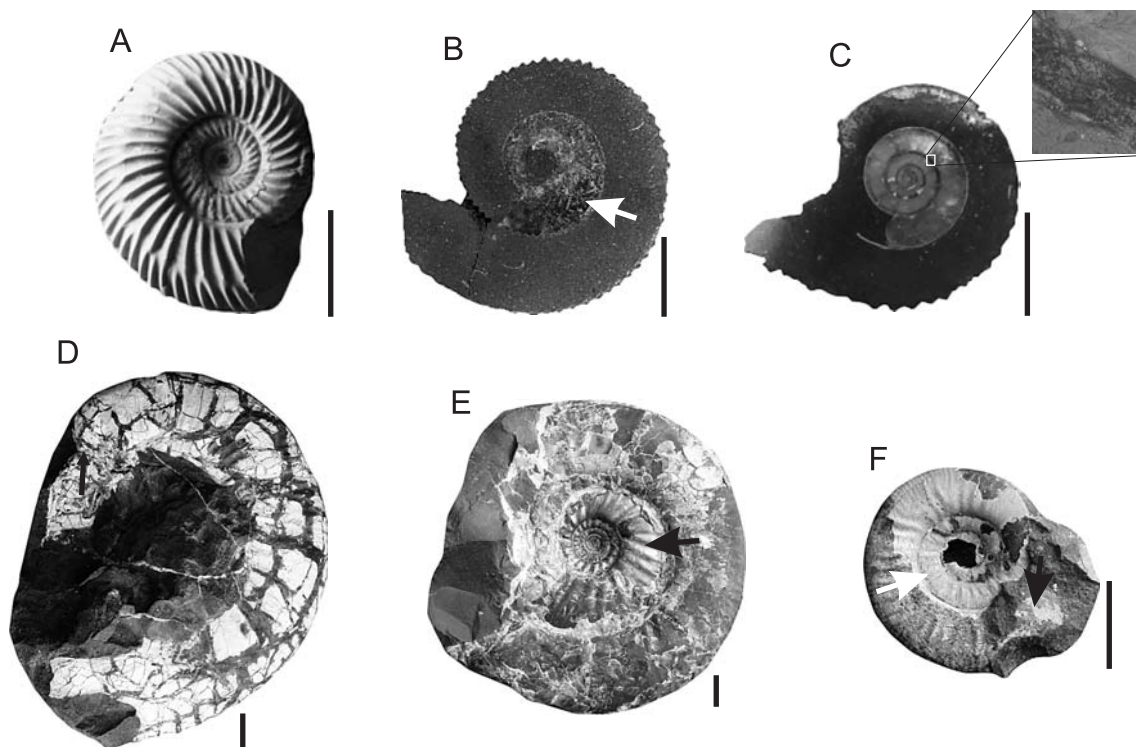
Fig. 5. Examples of preservation of ammonites from carbonate concretions
