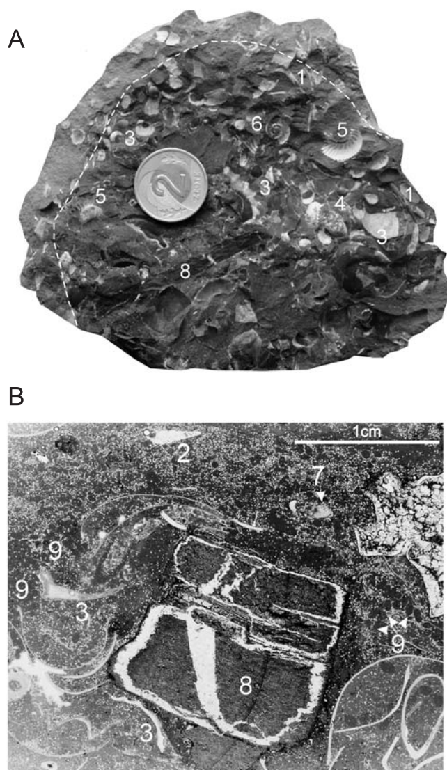
Fig. 2. A — broken carbonate concretion showing dense accumulation of fossils: the dashed line indicates the boundary between the outer and inner zone; B — thin-section showing a densely-packed shelly biomicrite microfacies
