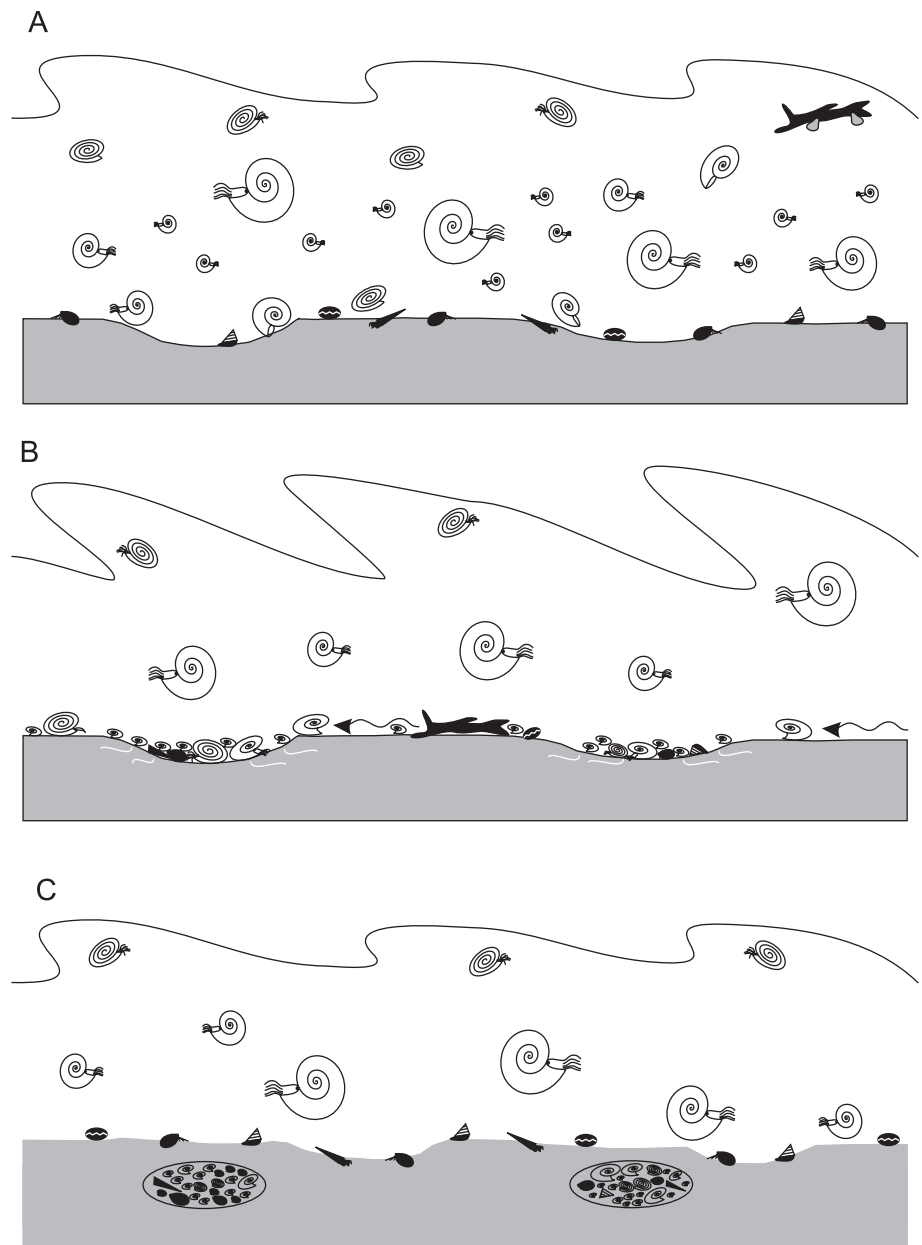
Fig. 7. Biostratinomic scenario describing accumulation of biological remains
