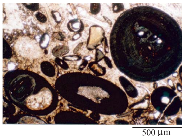
Fig. 4. Ferruginous grains in examined Famennian ironstones from the Howz-e-Dorah section (Fig. 3); the shell fragments as nuclei in some grains coated by concentric layers of the ferruginous cortex
