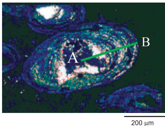
Fig. 4. Ferruginous grains in examined Famennian ironstones from the Howz-e-Dorah section (Fig. 3); the shell fragments as nuclei in some grains coated by concentric layers of the ferruginous cortex
