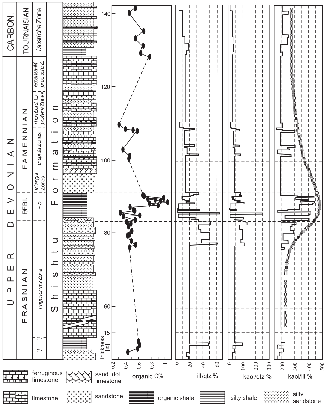
Fig. 3. Stratigraphy, organic carbon content and clay mineralogy in Howz-e-Dorah section
