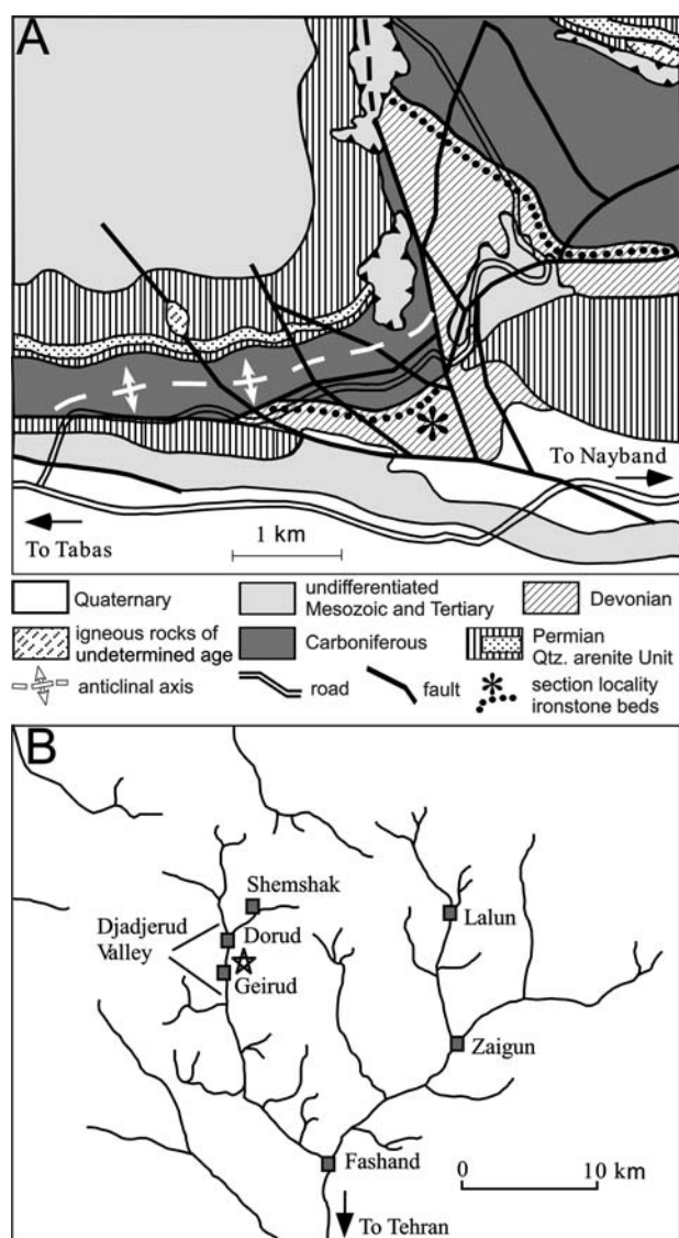
Fig. 2. A — geological map of Howz-e-Dorah area, east of Tabas (revised after Yazdi, 1999) with the location of studied section; B — sketch map of Djadjerud Valley with the location of Geirud section (shown by star)
