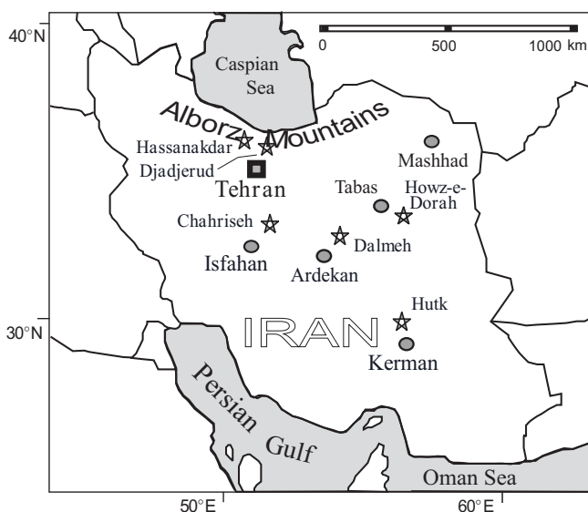
Fig. 1. Section localities in Iran (shown by stars)
