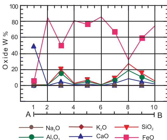
Fig. 5. EPMA scanned microphotograph and point analysis for determination of major oxides in cortex and nuclei in ferruginous grains of oolitic ironstone. Microphotograph shows distribution of Al in the grain. Ten point data from A to B represent the geochemical composition indicating aluminosilicates as main component. The core (point no. 1) contains higher CaO than cortex but no other oxides except for a few percent of FeO, indicating carbonate and probably a calcite shell fragment as nuclei
