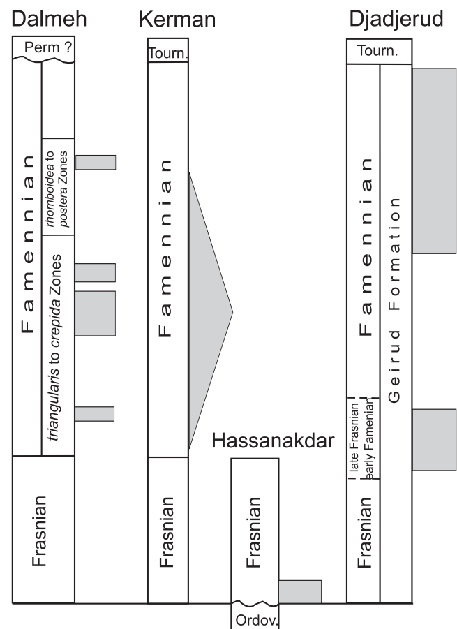
Fig. 6. Timing of basalt units in selected Iranian sections (see Fig. 1): central Iran, Ardekan area (conodont biostratigraphy after Hairapetian and Yazdi, 2003, fig. 3); southeastern Iran, Kerman area (after Wendt et al. , 2002, fig. 4, Zone C); northern Iran, Central Alborz, Hassanakdar area (dated by palynomorphs, after Ghavidel-Syooki, 1994, fig. 2); northern Iran, Central Alborz, Djadjerud Valley (Mahmudy Gharai, 2002)
