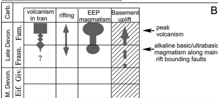
Fig. 7. A — in grey — distribution of the main areas of Late Devonian rifting and magmatism in the East European Platform (EEP; revised after Wilson and Lyashkevich, 1996, fig. 1) and the North Gondwanan domain; PDD — Pripyat-Dnepr-Donets Rift; B — timing of rifting and magmatism in Iran (based on Figure 6) and East European Platform (EEP) during Late Devonian (revised after Wilson and Lyashkevich, 1996)
