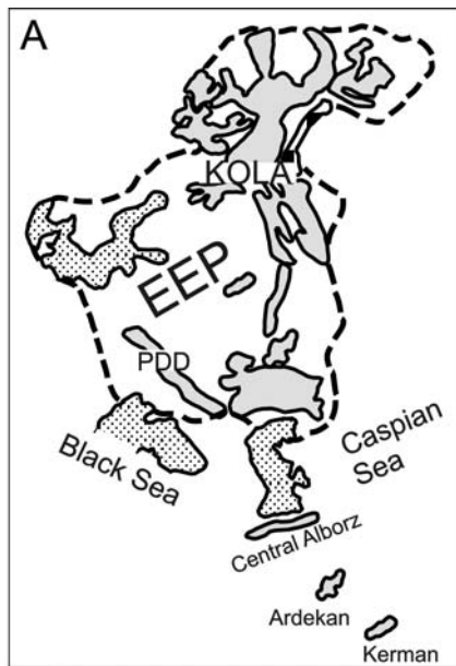
Fig. 7. A — in grey — distribution of the main areas of Late Devonian rifting and magmatism in the East European Platform (EEP; revised after Wilson and Lyashkevich, 1996, fig. 1) and the North Gondwanan domain; PDD — Pripyat-Dnepr-Donets Rift; B — timing of rifting and magmatism in Iran (based on Figure 6) and East European Platform (EEP) during Late Devonian (revised after Wilson and Lyashkevich, 1996)
