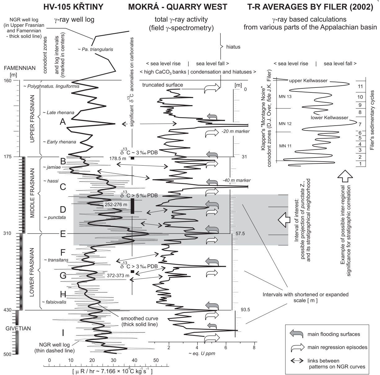
Fig. 2. Comparison of the Křtiny HV-105 borehole and Mokrá — quarry west; natural \gamma -ray records
