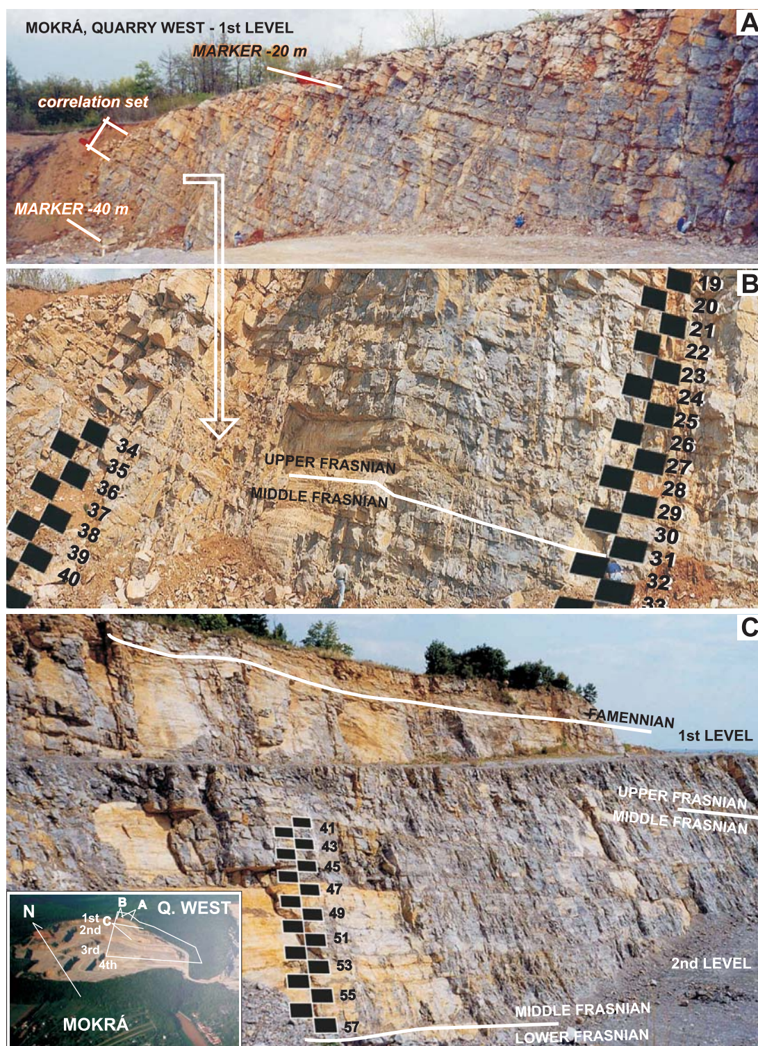
Fig. 5. The eastern upper part of Mokrý — quarry west (field situation)
