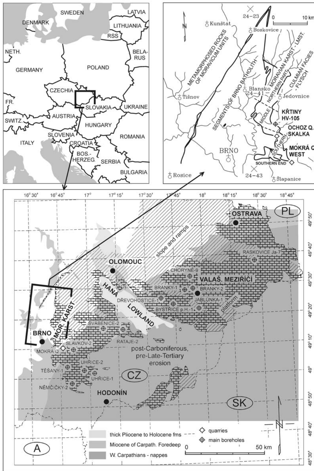
Fig. 1. Location of sections studied in Moravia, E part of the Czech Republic.
