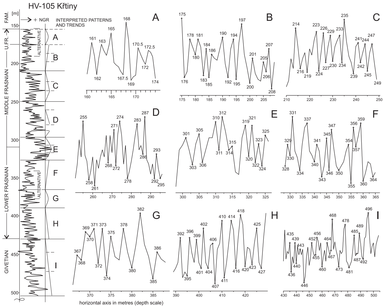
Fig. 3. Discerned NGR log intervals, HV-105 Křtiny borehole
