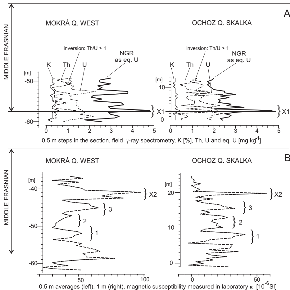
Fig. 4. Diagnostic patterns for search of punctata stratigraphic equivalents in coral-stromatoporoid limestones of carbonate platforms
