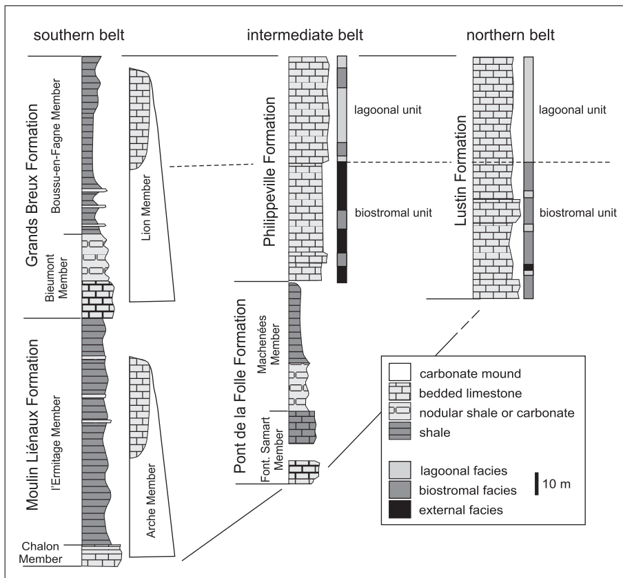
Fig. 3. Correlation of synthetic sections across the middle Frasnian carbonate platform in Belgium, with lithostratigraphic units and facies types
