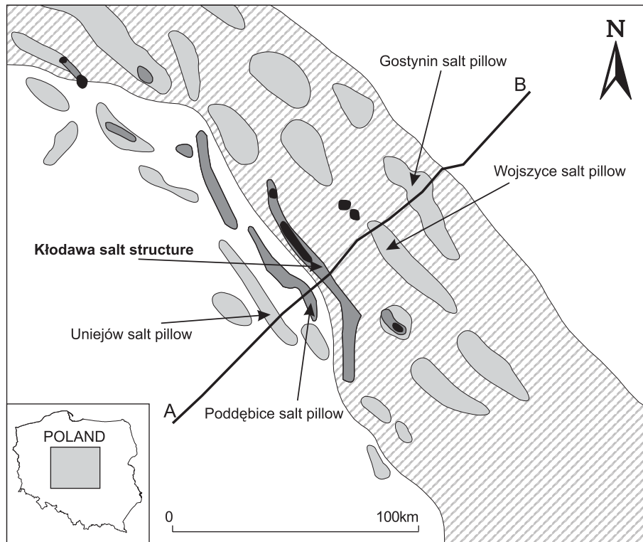
Fig. 2. Distribution of salt structures within the central (Kuiavian) part of the Mid-Polish Trough (from Dadlez and Marek, 1998, simplified)
