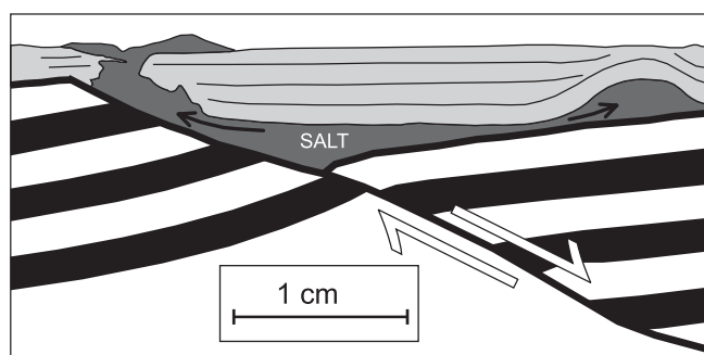
Fig. 9. Basement faulting, salt movements and deposition — results of centrifuge modelling; note movement of the salt along the hangingwall towards the salt pillow, and towards the footwall, towards the salt diapir (from Koyi et al. , 1993); compare to the model of the Triassic evolution of the Kłodawa salt structure (Fig. 7)
