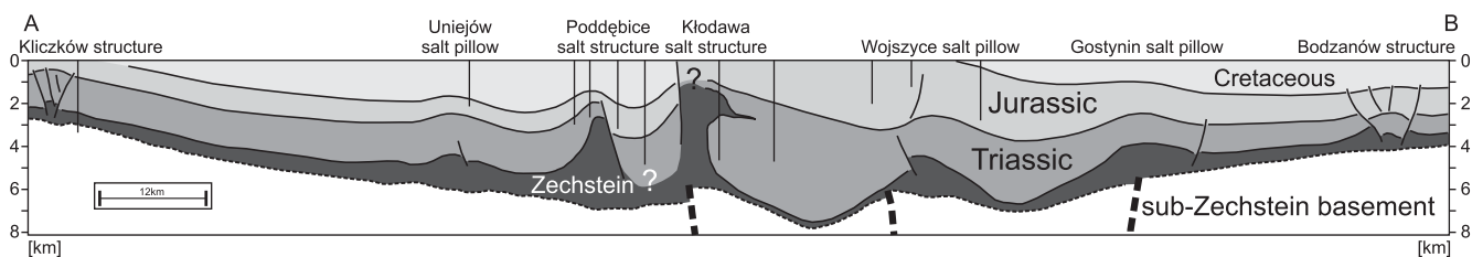
Fig. 4. Interpreted regional seismic profile from the central part of the Mid-Polish Trough, crossing the Kłodawa salt structure
