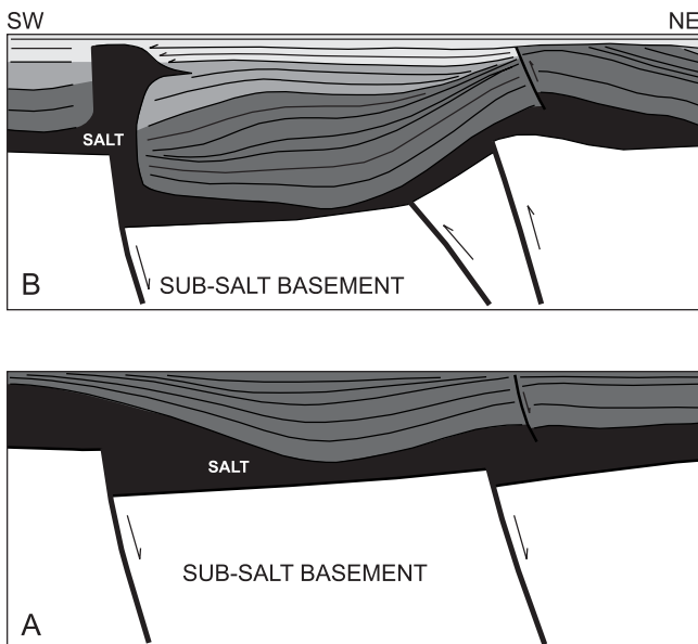
Fig. 7. A qualitative model of the Triassic development of the Kłodawa salt structure and surrounding depositional systems
