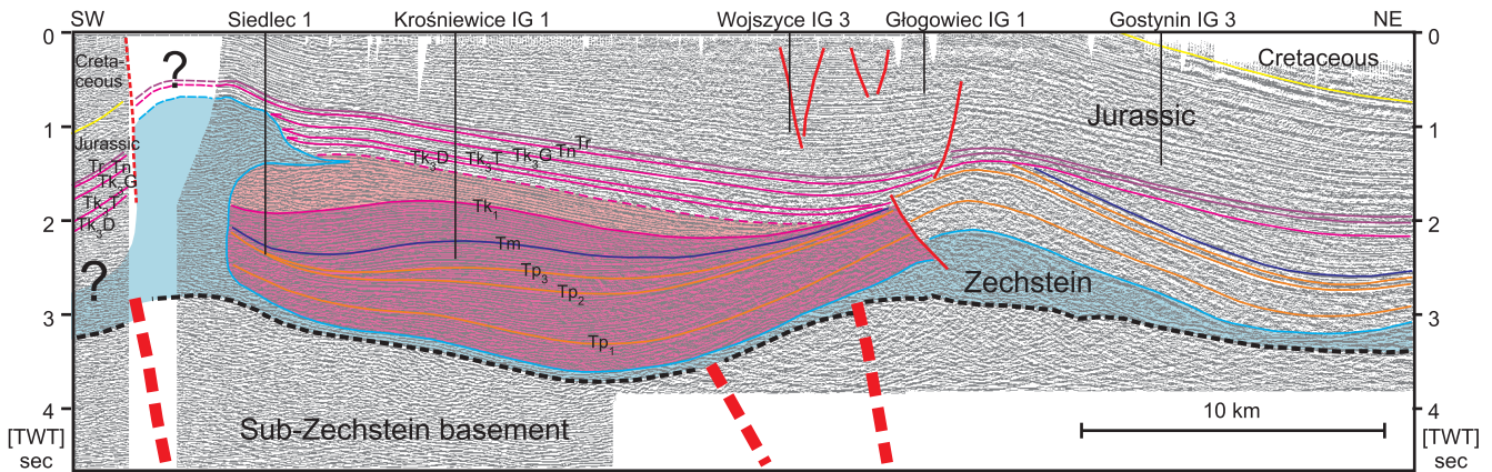
Fig. 5. Interpreted part of regional seismic profile crossing the Kłodawa salt structure
