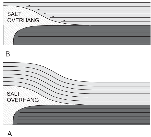
Fig. 8. Alternative models of a relationship between the salt overhang and overlying deposits
