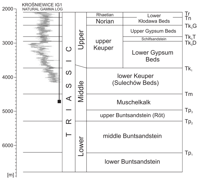
Fig. 3. Triassic lithostratigraphy (after Gajewska in: Marek and Pajchlowa, 1997, simplified) and the Triassic thickness distribution along and below the Krośniewice IG 1 borehole
