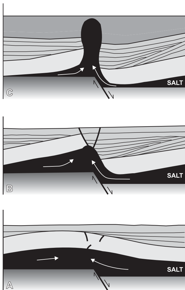
Fig. 1. Schematic diagram (based on results of analogue modelling) showing different stages of salt structure evolution above faulted basement (from Koyi et al. , 1993, slightly modified)
