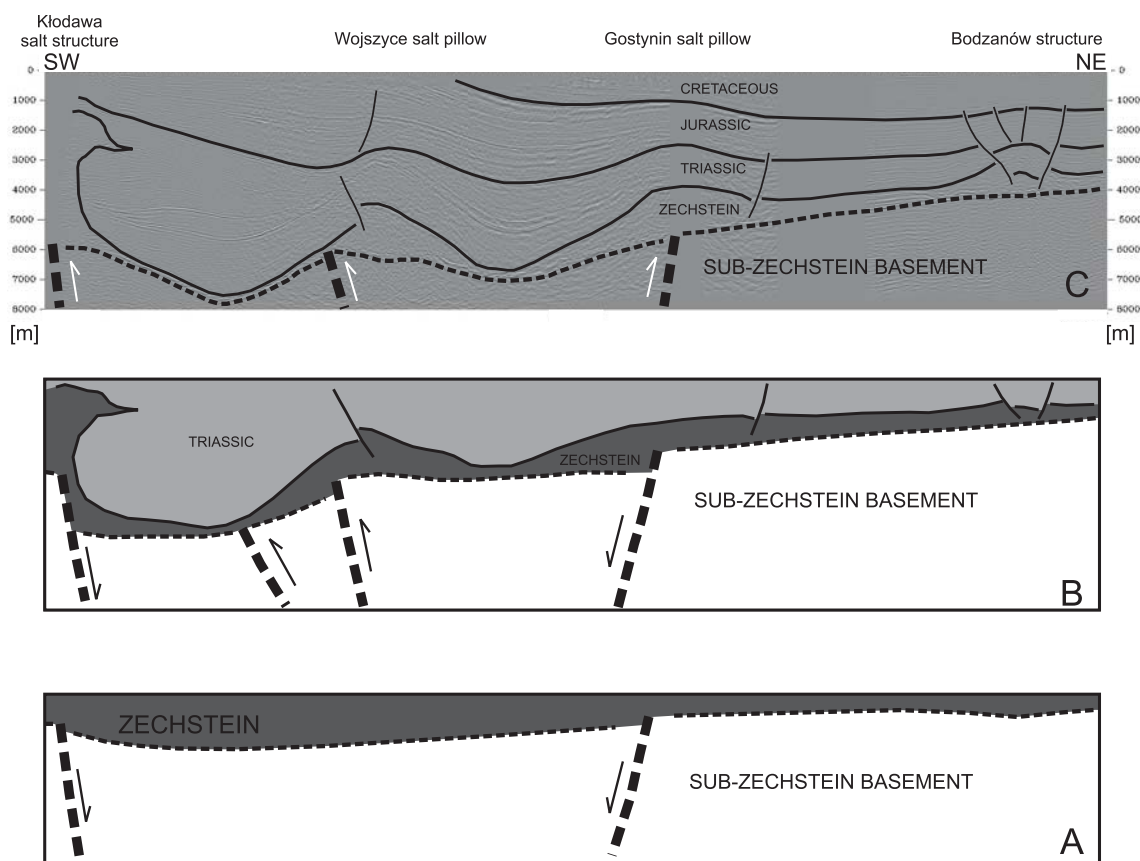
Fig. 6. Late Permian (A) and Late Triassic (B) qualitative (not balanced, without decompaction) reconstructions, and present-day (C) upper crustal configuration along the central part of the regional seismic profile from Figure 4
