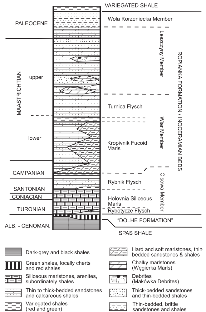
Fig. 2. Generalised stratigraphic log of the Albian–Paleocene of the Skole Nappe of the Polish Carpathians, slightly modified after Kotlarczyk (1988)
