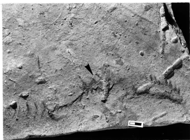
Fig. 42. Form C (arrowed)
