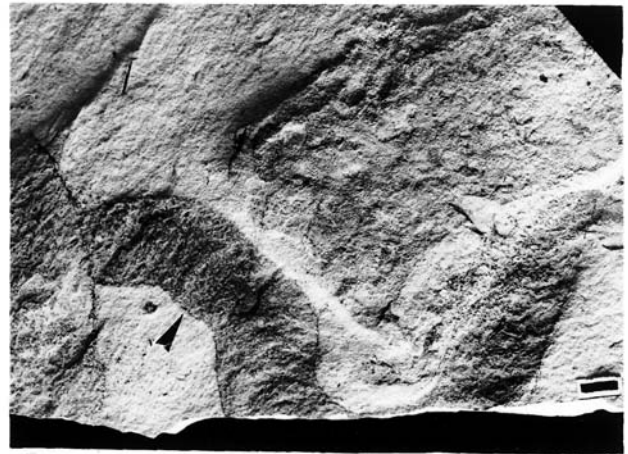
Fig. 29. Indistinctly meniscate endichnial structure (arrowed) resembling Scolicia ?plana in winding style and width;
