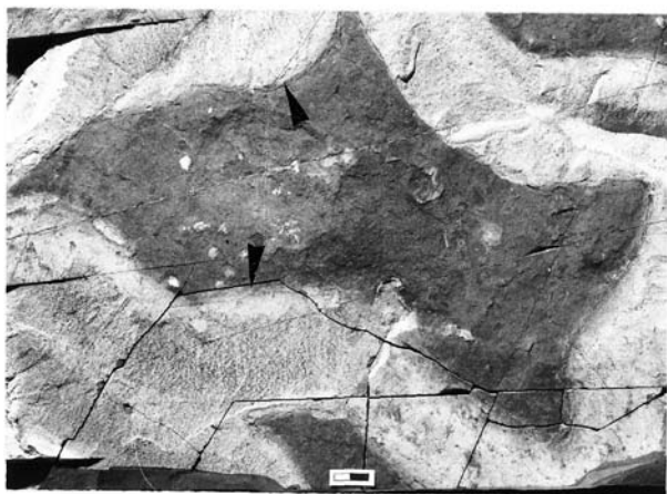
Fig. 31. Scolicia isp. A (arrowed)
