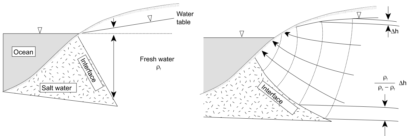
Fig. 1. Shape of freshwater/seawater interface, Gyben-Heltzberg interface (L) and actual interface in the condition of flowing groundwater (R) (after Bower, 1978)
